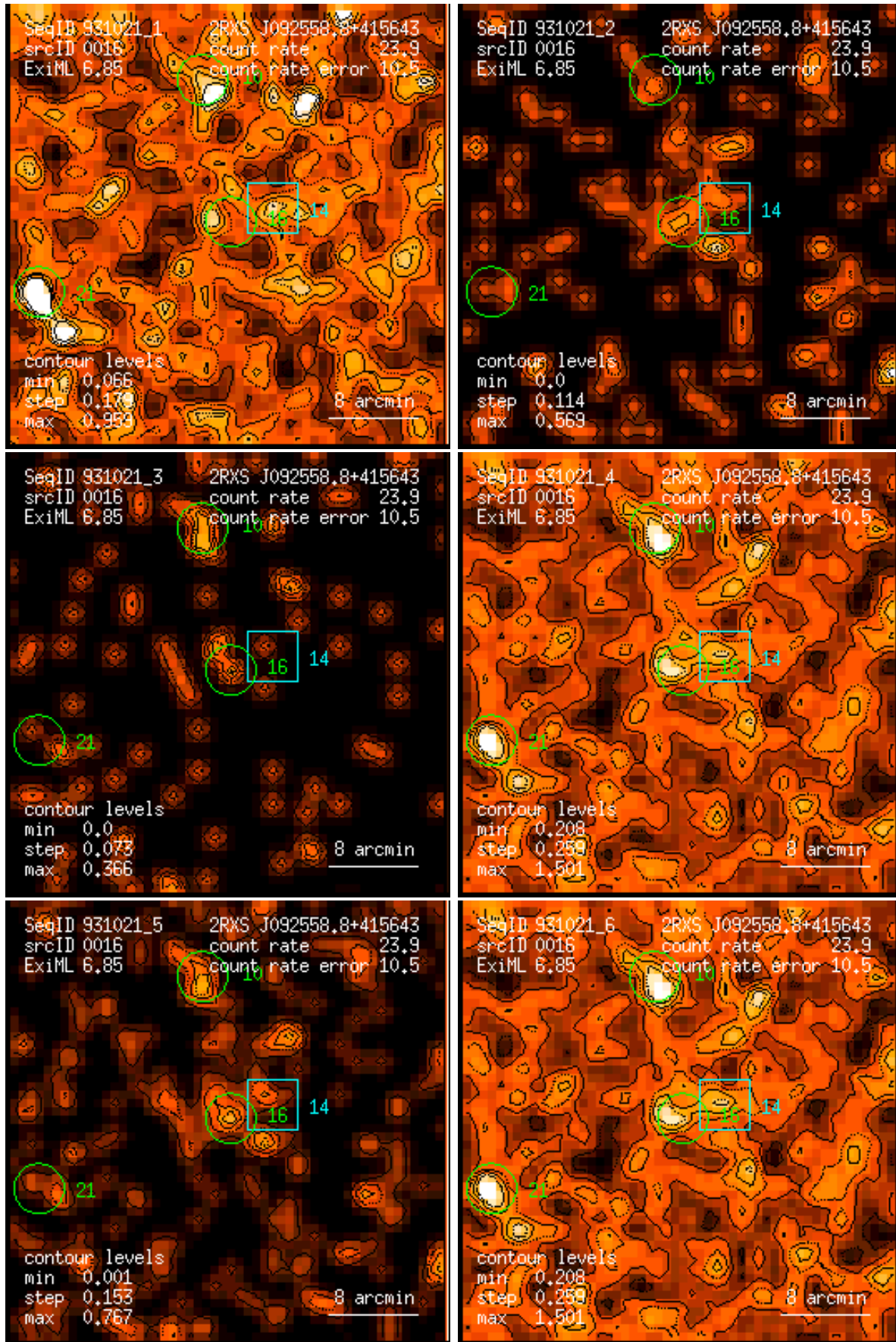
Figure 16: RASS 931021: detection 0016: band rate images, Gaussian filter: (1) PSPC channels 11 – 41, (2) 52 – 90, (3) 91 – 201, (4) 11 – 235, (5) 52 – 201, (6) 11 – 201. Broad band rates in counts/ks. Band rate contour levels in counts/ks/arcmin 2 .
