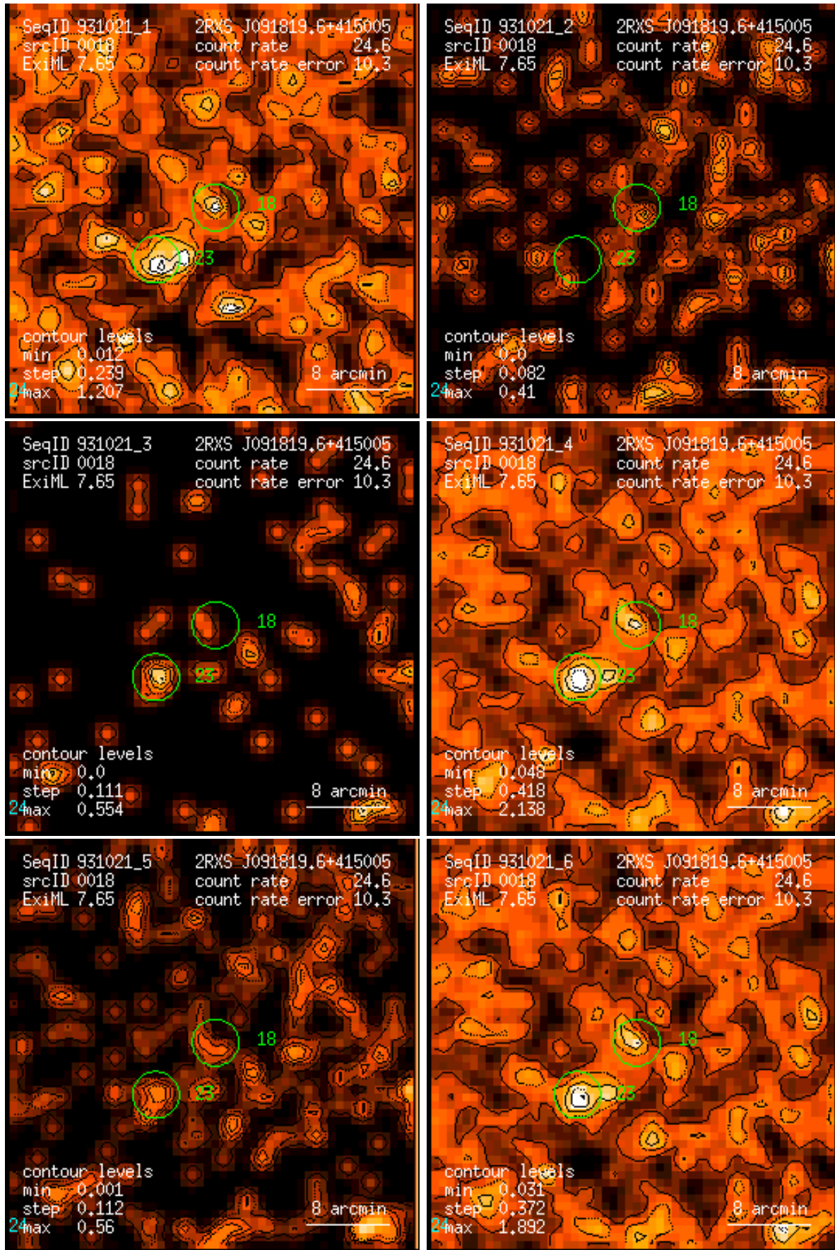
Figure 18: RASS 931021: detection 0018: band rate images, Gaussian filter: (1) PSPC channels 11 – 41, (2) 52 – 90, (3) 91 – 201, (4) 11 – 235, (5) 52 – 201, (6) 11 – 201. Broad band rates in counts/ks. Band rate contour levels in counts/ks/arcmin 2 .
