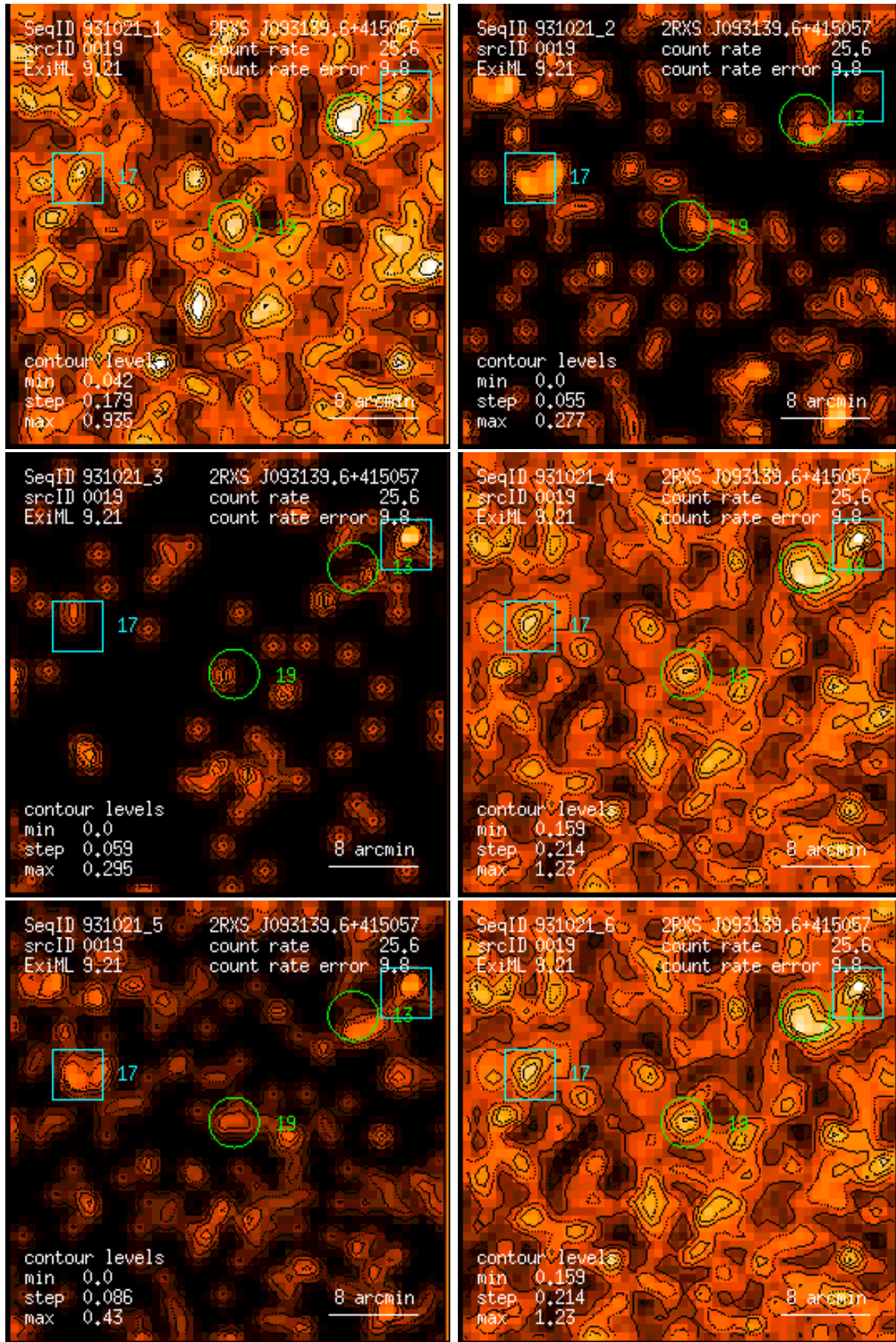
Figure 19: RASS 931021: detection 0019: band rate images, Gaussian filter: (1) PSPC channels 11 – 41, (2) 52 – 90, (3) 91 – 201, (4) 11 – 235, (5) 52 – 201, (6) 11 – 201. Broad band rates in counts/ks. Band rate contour levels in counts/ks/arcmin 2 .
