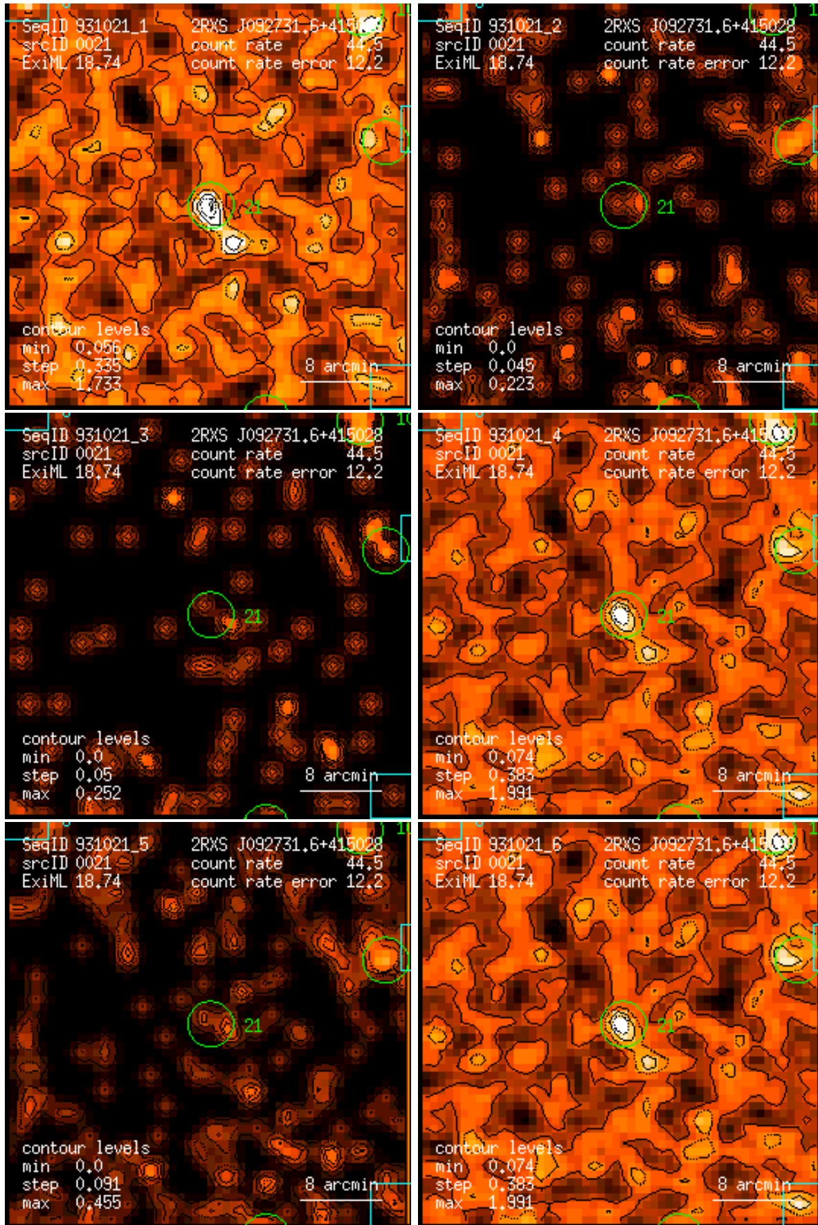
Figure 21: RASS 931021: detection 0021: band rate images, Gaussian filter: (1) PSPC channels 11 – 41, (2) 52 – 90, (3) 91 – 201, (4) 11 – 235, (5) 52 – 201, (6) 11 – 201. Broad band rates in counts/ks. Band rate contour levels in counts/ks/arcmin 2 .
