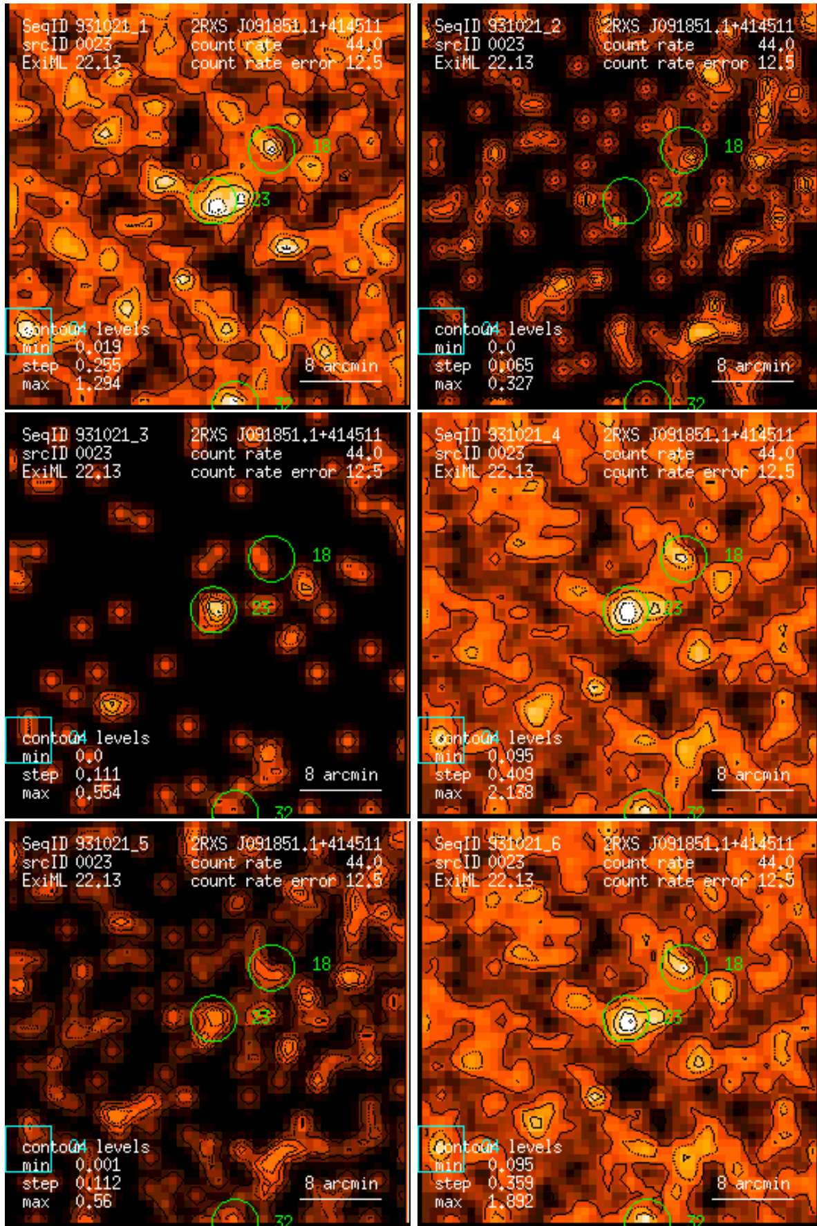
Figure 23: RASS 931021: detection 0023: band rate images, Gaussian filter: (1) PSPC channels 11 – 41, (2) 52 – 90, (3) 91 – 201, (4) 11 – 235, (5) 52 – 201, (6) 11 – 201. Broad band rates in counts/ks. Band rate contour levels in counts/ks/arcmin 2 .
