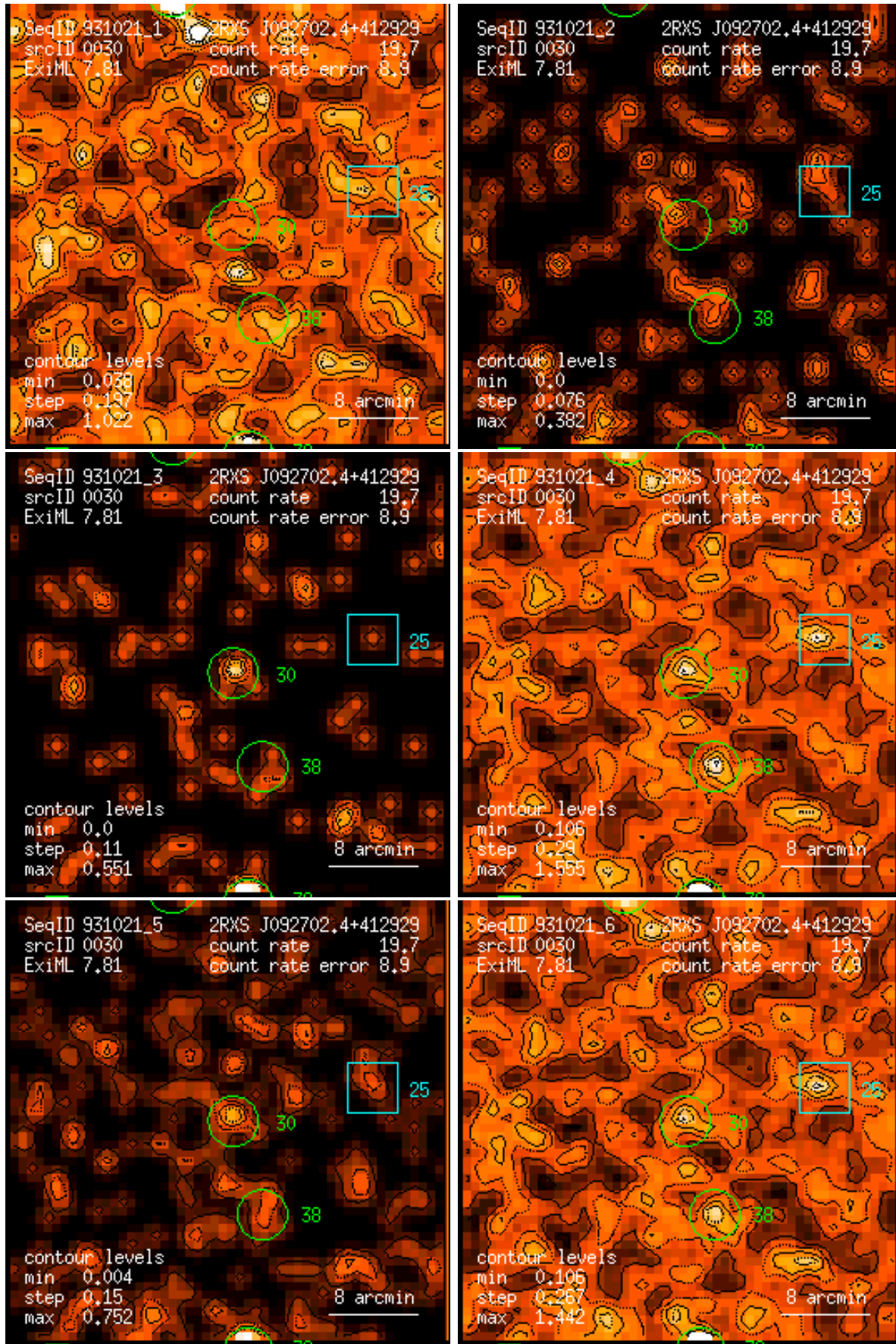
Figure 30: RASS 931021: detection 0030: band rate images, Gaussian filter: (1) PSPC channels 11 – 41, (2) 52 – 90, (3) 91 – 201, (4) 11 – 235, (5) 52 – 201, (6) 11 – 201. Broad band rates in counts/ks. Band rate contour levels in counts/ks/arcmin 2 .
