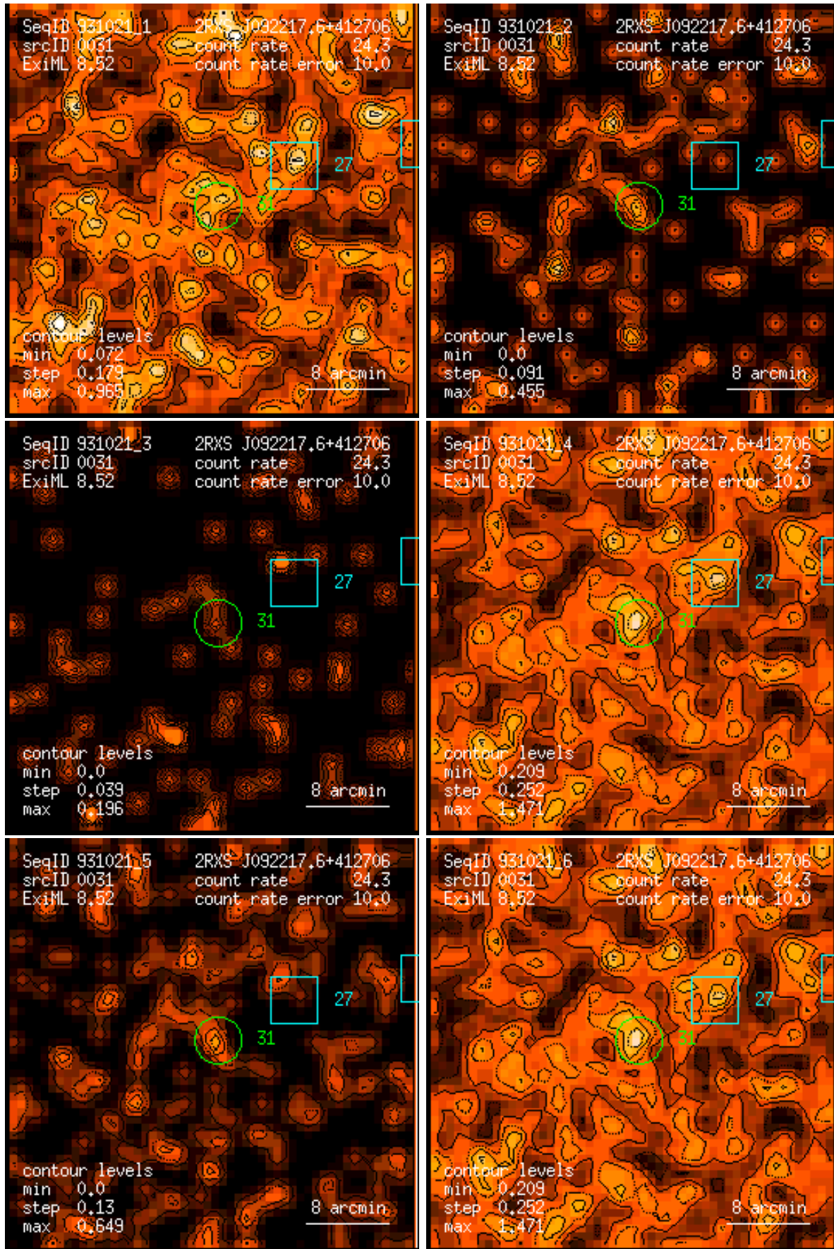
Figure 31: RASS 931021: detection 0031: band rate images, Gaussian filter: (1) PSPC channels 11 – 41, (2) 52 – 90, (3) 91 – 201, (4) 11 – 235, (5) 52 – 201, (6) 11 – 201. Broad band rates in counts/ks. Band rate contour levels in counts/ks/arcmin 2 .
