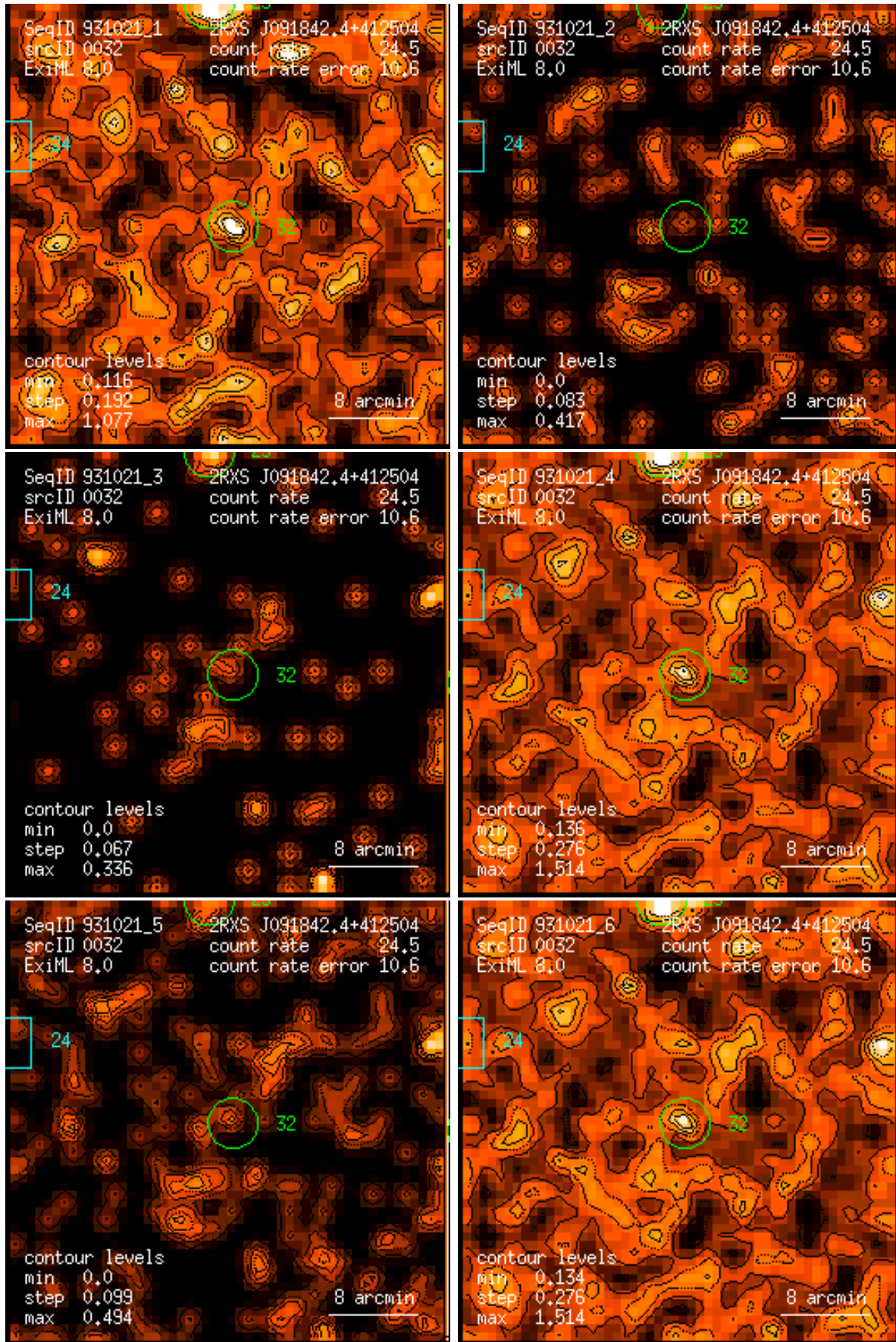
Figure 32: RASS 931021: detection 0032: band rate images, Gaussian filter: (1) PSPC channels 11 – 41, (2) 52 – 90, (3) 91 – 201, (4) 11 – 235, (5) 52 – 201, (6) 11 – 201. Broad band rates in counts/ks. Band rate contour levels in counts/ks/arcmin 2 .
