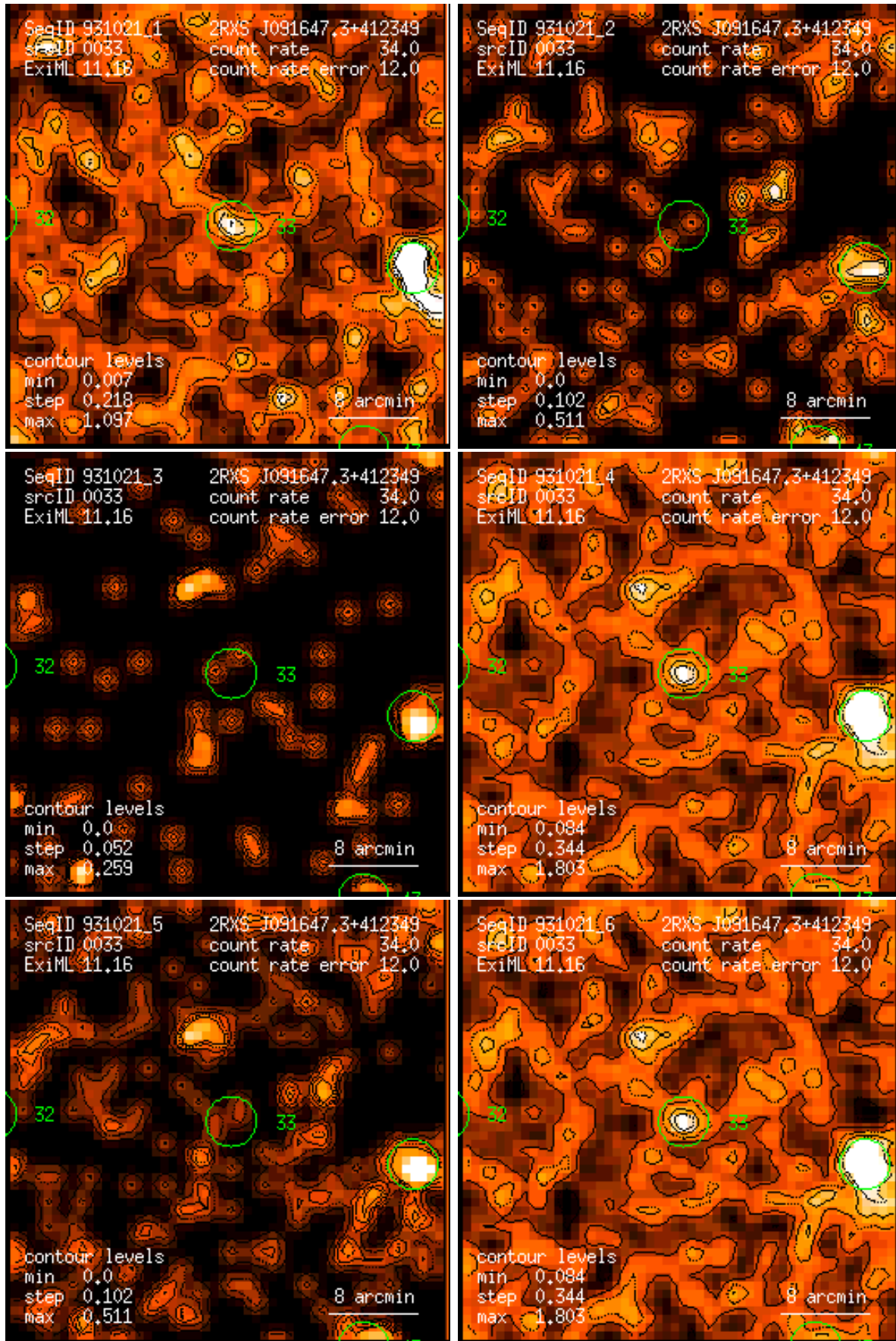
Figure 33: RASS 931021: detection 0033: band rate images, Gaussian filter: (1) PSPC channels 11 – 41, (2) 52 – 90, (3) 91 – 201, (4) 11 – 235, (5) 52 – 201, (6) 11 – 201. Broad band rates in counts/ks. Band rate contour levels in counts/ks/arcmin 2 .
