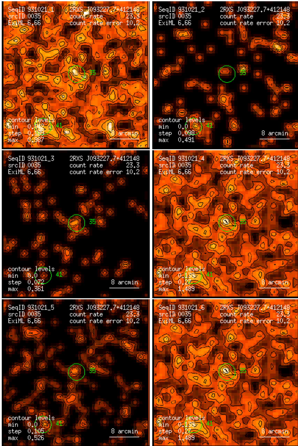
Figure 35: RASS 931021: detection 0035: band rate images, Gaussian filter: (1) PSPC channels 11 – 41, (2) 52 – 90, (3) 91 – 201, (4) 11 – 235, (5) 52 – 201, (6) 11 – 201. Broad band rates in counts/ks. Band rate contour levels in counts/ks/arcmin 2 .
