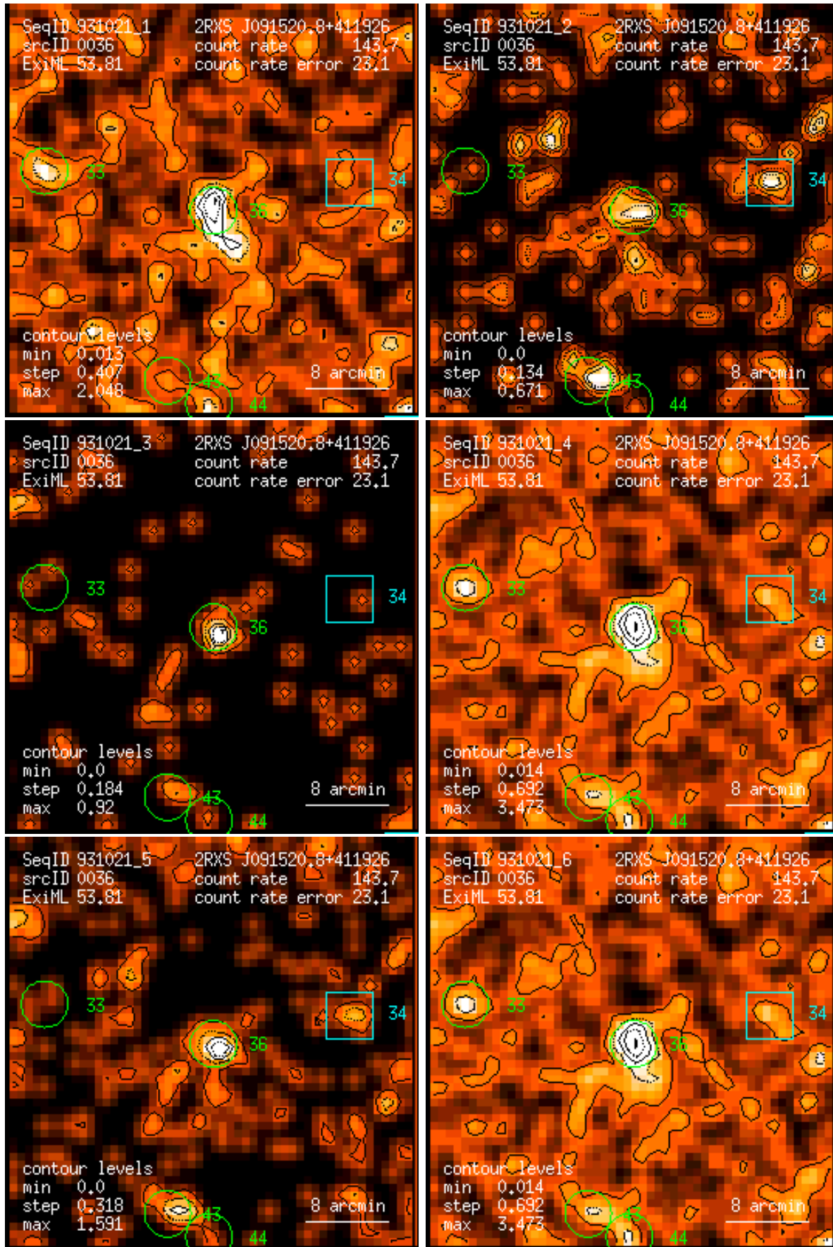
Figure 36: RASS 931021: detection 0036: band rate images, Gaussian filter: (1) PSPC channels 11 – 41, (2) 52 – 90, (3) 91 – 201, (4) 11 – 235, (5) 52 – 201, (6) 11 – 201. Broad band rates in counts/ks. Band rate contour levels in counts/ks/arcmin 2 .
