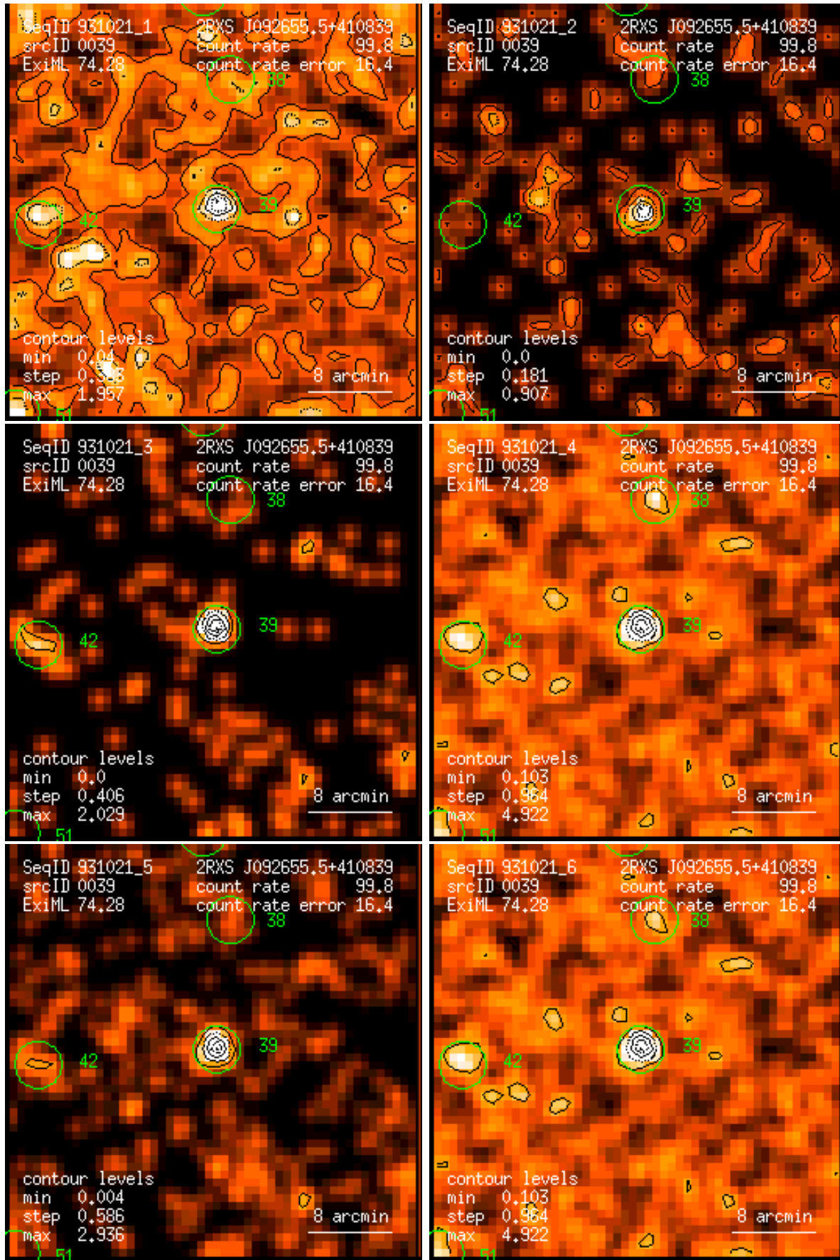
Figure 39: RASS 931021: detection 0039: band rate images, Gaussian filter: (1) PSPC channels 11 – 41, (2) 52 – 90, (3) 91 – 201, (4) 11 – 235, (5) 52 – 201, (6) 11 – 201. Broad band rates in counts/ks. Band rate contour levels in counts/ks/arcmin 2 .
