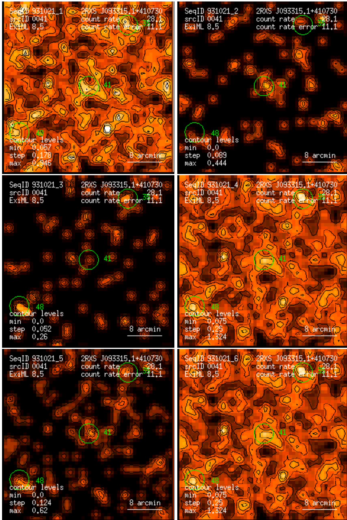
Figure 41: RASS 931021: detection 0041: band rate images, Gaussian filter: (1) PSPC channels 11 – 41, (2) 52 – 90, (3) 91 – 201, (4) 11 – 235, (5) 52 – 201, (6) 11 – 201. Broad band rates in counts/ks. Band rate contour levels in counts/ks/arcmin 2 .
