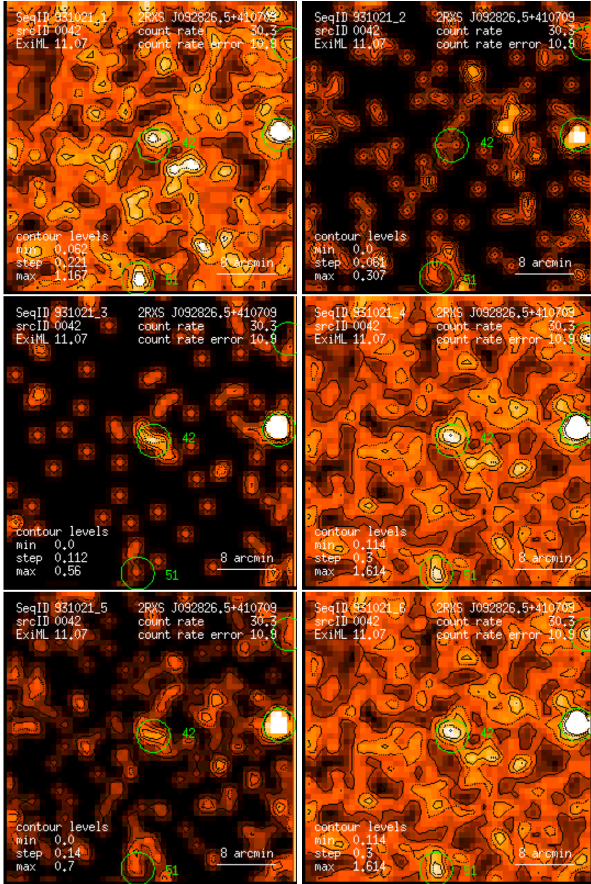
Figure 42: RASS 931021: detection 0042: band rate images, Gaussian filter: (1) PSPC channels 11 – 41, (2) 52 – 90, (3) 91 – 201, (4) 11 – 235, (5) 52 – 201, (6) 11 – 201. Broad band rates in counts/ks. Band rate contour levels in counts/ks/arcmin 2 .
