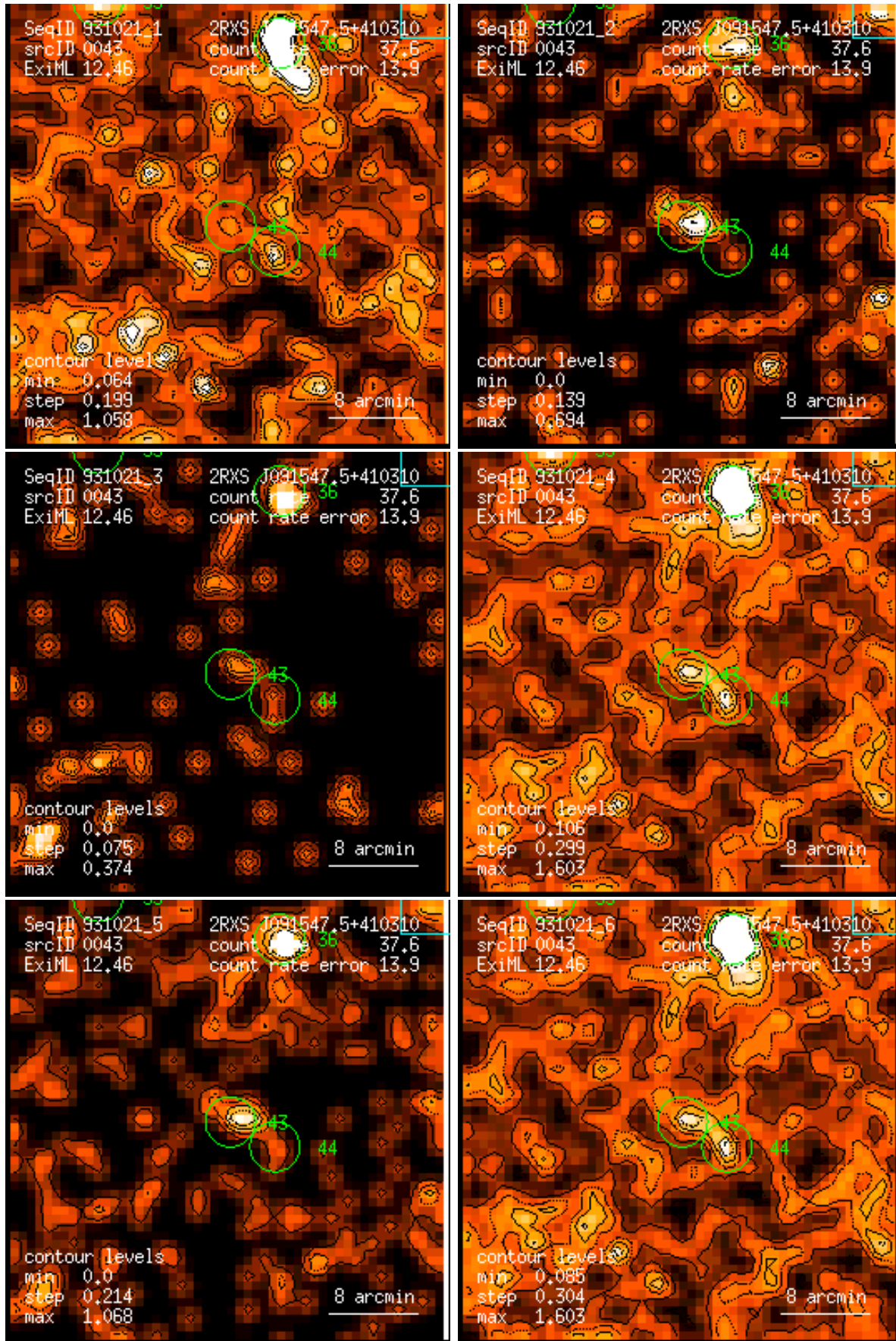
Figure 43: RASS 931021: detection 0043: band rate images, Gaussian filter: (1) PSPC channels 11 – 41, (2) 52 – 90, (3) 91 – 201, (4) 11 – 235, (5) 52 – 201, (6) 11 – 201. Broad band rates in counts/ks. Band rate contour levels in counts/ks/arcmin 2 .
