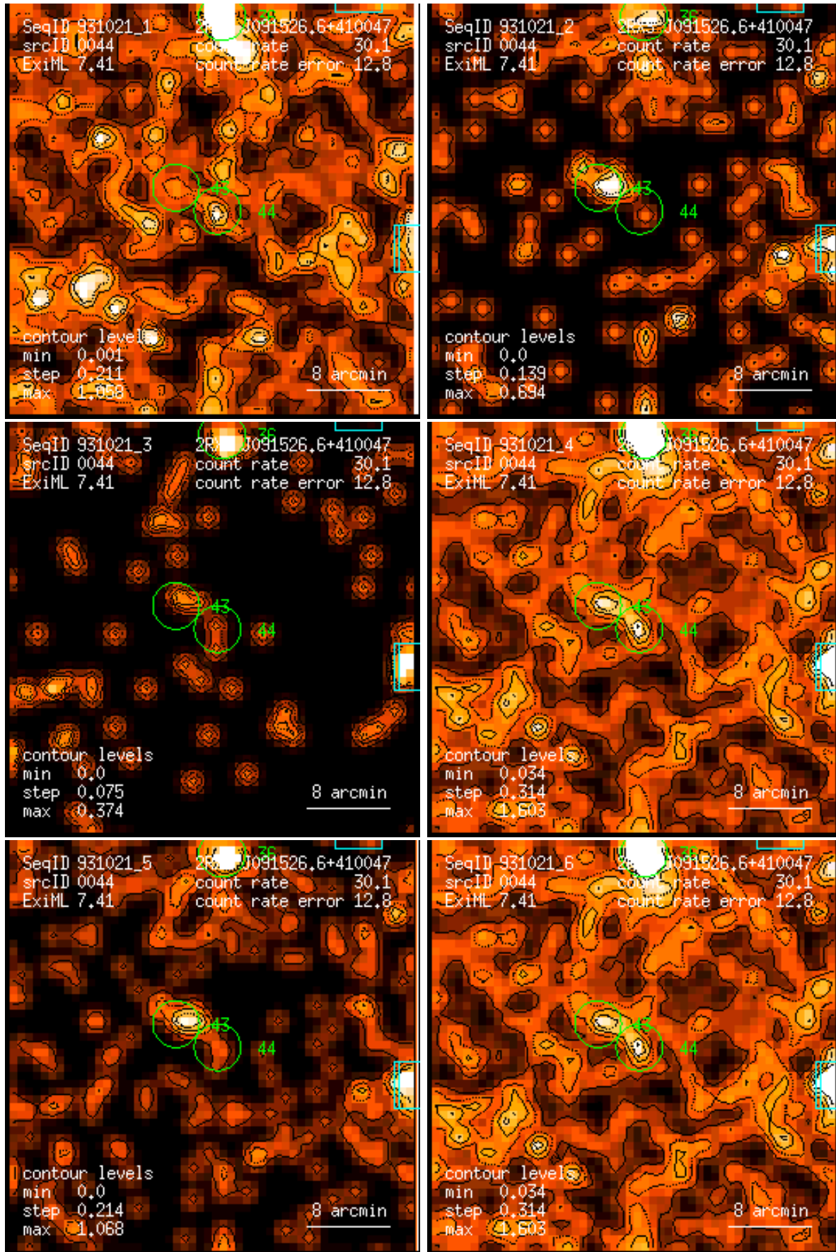
Figure 44: RASS 931021: detection 0044: band rate images, Gaussian filter: (1) PSPC channels 11 – 41, (2) 52 – 90, (3) 91 – 201, (4) 11 – 235, (5) 52 – 201, (6) 11 – 201. Broad band rates in counts/ks. Band rate contour levels in counts/ks/arcmin 2 .
