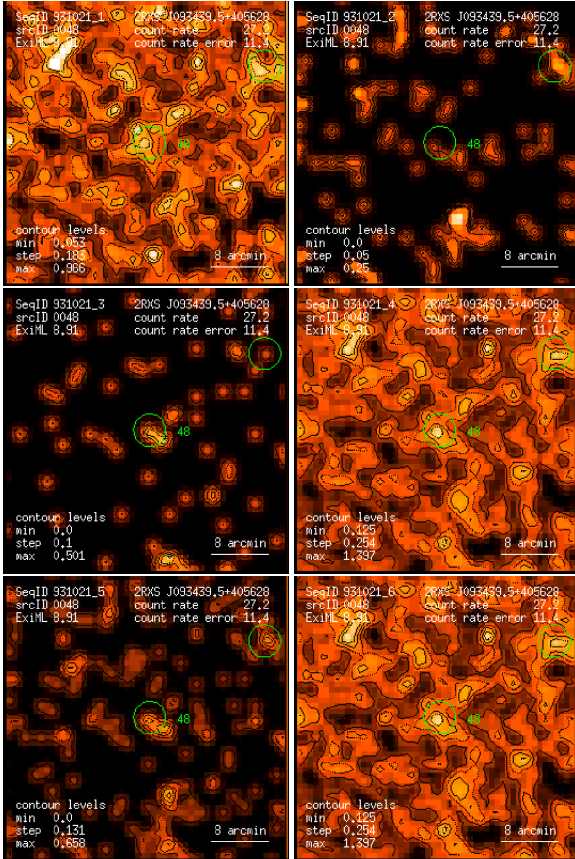
Figure 48: RASS 931021: detection 0048: band rate images, Gaussian filter: (1) PSPC channels 11 – 41, (2) 52 – 90, (3) 91 – 201, (4) 11 – 235, (5) 52 – 201, (6) 11 – 201. Broad band rates in counts/ks. Band rate contour levels in counts/ks/arcmin 2 .
