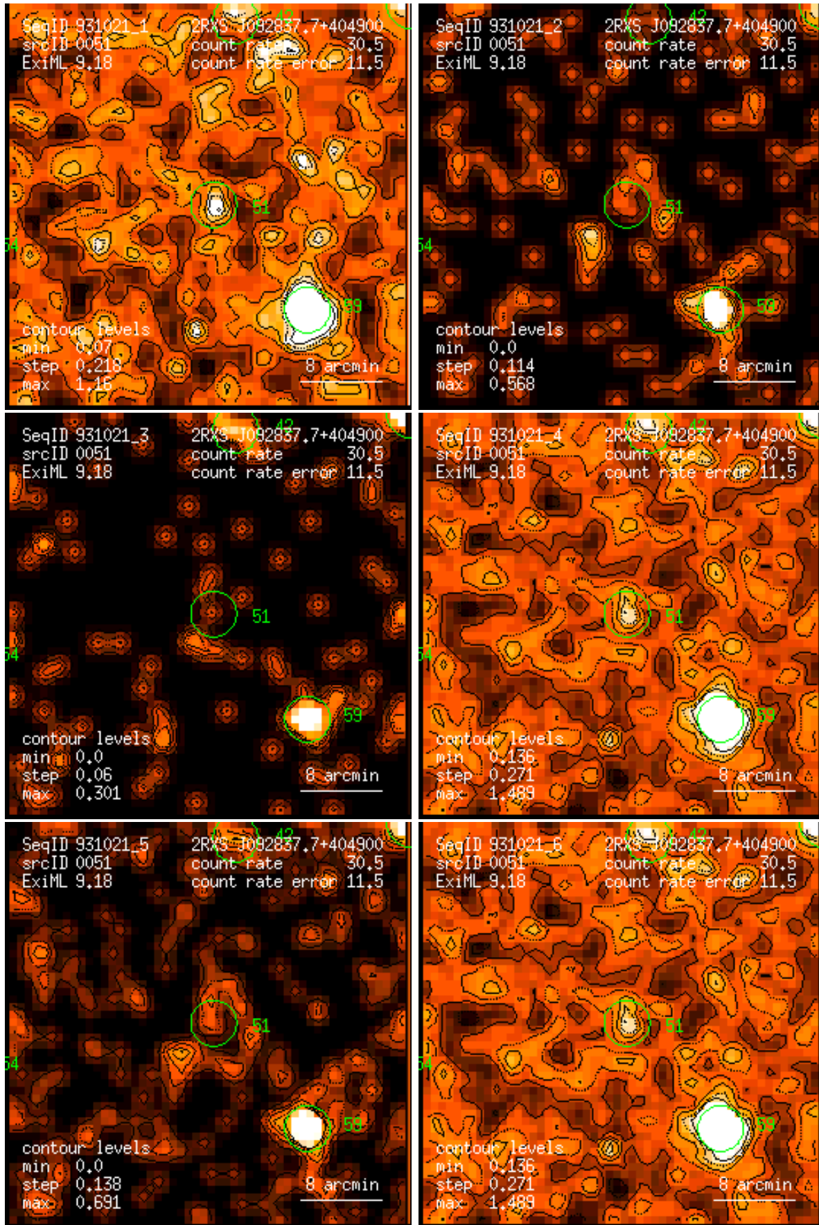
Figure 51: RASS 931021: detection 0051: band rate images, Gaussian filter: (1) PSPC channels 11 – 41, (2) 52 – 90, (3) 91 – 201, (4) 11 – 235, (5) 52 – 201, (6) 11 – 201. Broad band rates in counts/ks. Band rate contour levels in counts/ks/arcmin 2 .
