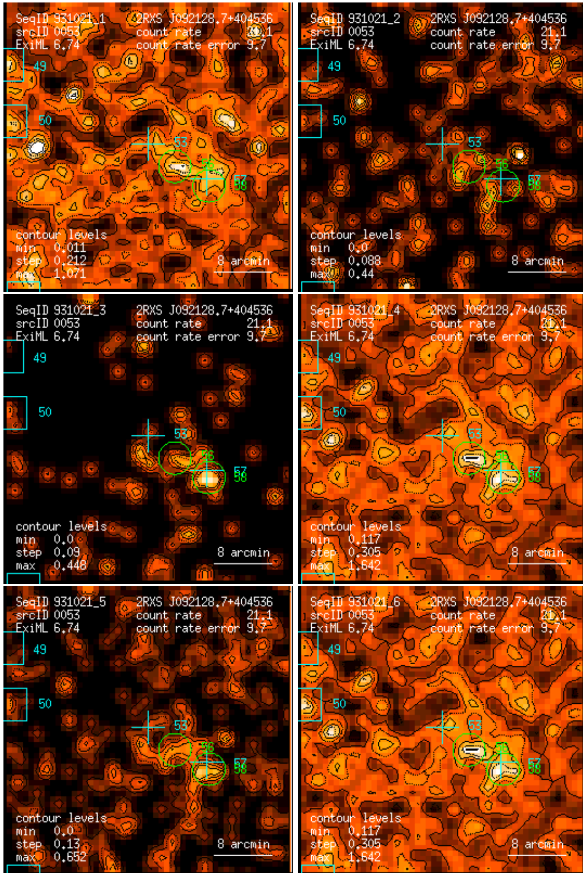
Figure 53: RASS 931021: detection 0053: band rate images, Gaussian filter: (1) PSPC channels 11 – 41, (2) 52 – 90, (3) 91 – 201, (4) 11 – 235, (5) 52 – 201, (6) 11 – 201. Broad band rates in counts/ks. Band rate contour levels in counts/ks/arcmin 2 .
