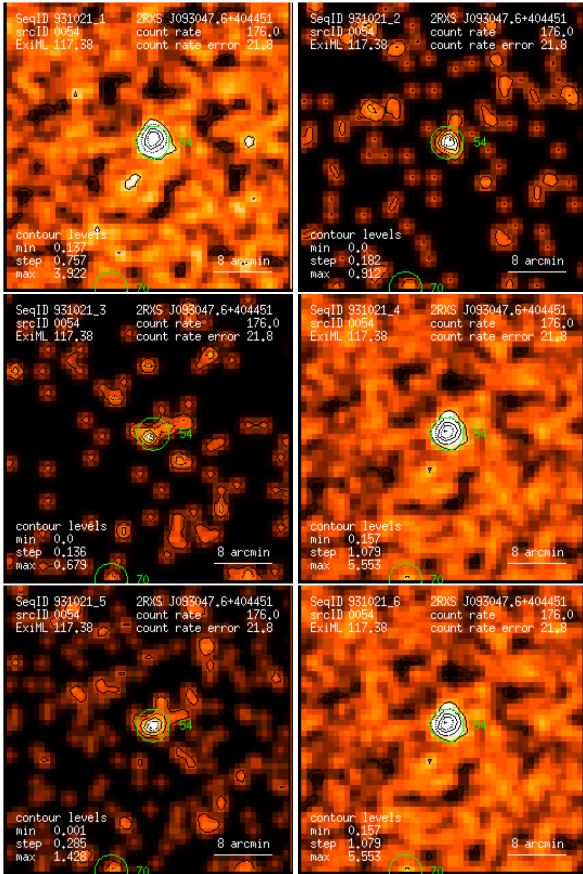
Figure 54: RASS 931021: detection 0054: band rate images, Gaussian filter: (1) PSPC channels 11 – 41, (2) 52 – 90, (3) 91 – 201, (4) 11 – 235, (5) 52 – 201, (6) 11 – 201. Broad band rates in counts/ks. Band rate contour levels in counts/ks/arcmin 2 .
