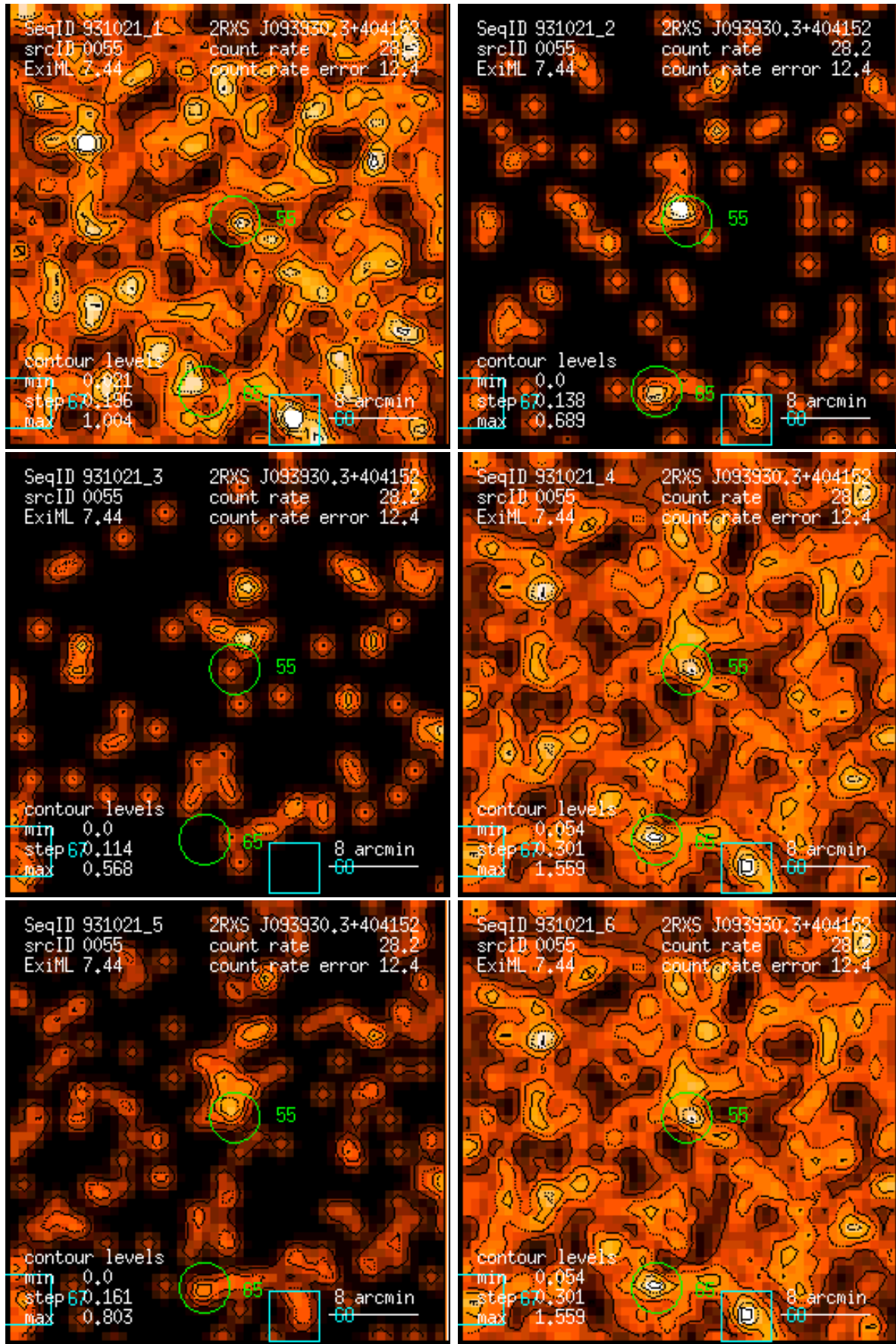
Figure 55: RASS 931021: detection 0055: band rate images, Gaussian filter: (1) PSPC channels 11 – 41, (2) 52 – 90, (3) 91 – 201, (4) 11 – 235, (5) 52 – 201, (6) 11 – 201. Broad band rates in counts/ks. Band rate contour levels in counts/ks/arcmin 2 .
