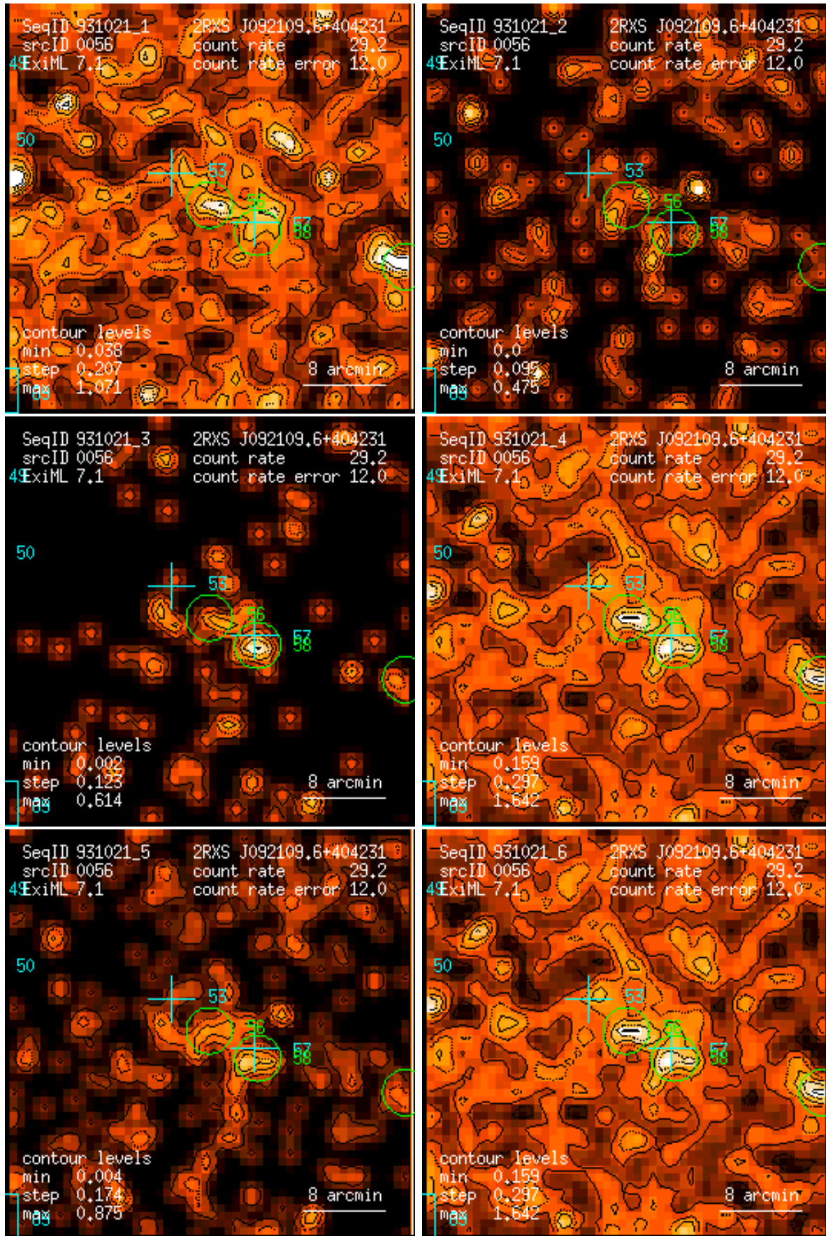
Figure 56: RASS 931021: detection 0056: band rate images, Gaussian filter: (1) PSPC channels 11 – 41, (2) 52 – 90, (3) 91 – 201, (4) 11 – 235, (5) 52 – 201, (6) 11 – 201. Broad band rates in counts/ks. Band rate contour levels in counts/ks/arcmin 2 .
