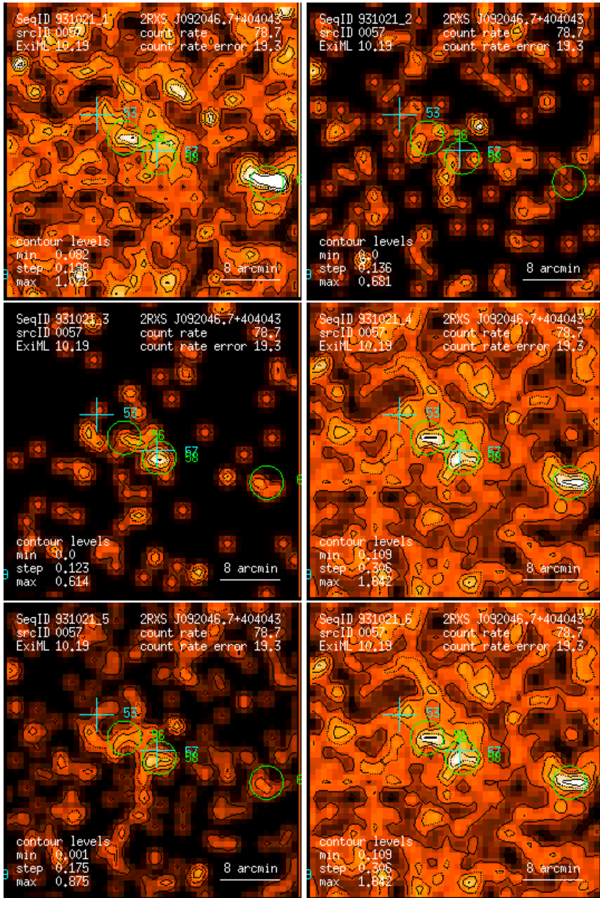
Figure 57: RASS 931021: detection 0057: band rate images, Gaussian filter: (1) PSPC channels 11 – 41, (2) 52 – 90, (3) 91 – 201, (4) 11 – 235, (5) 52 – 201, (6) 11 – 201. Broad band rates in counts/ks. Band rate contour levels in counts/ks/arcmin 2 .
