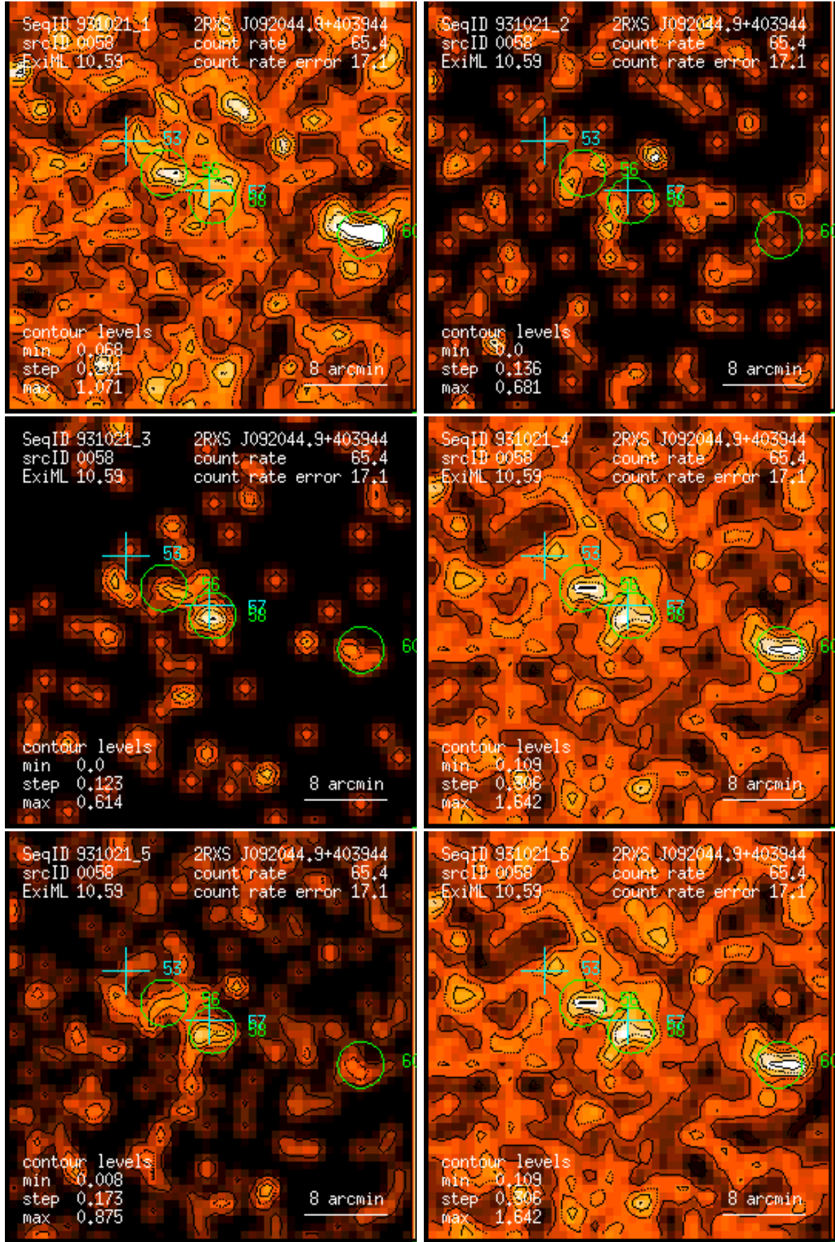
Figure 58: RASS 931021: detection 0058: band rate images, Gaussian filter: (1) PSPC channels 11 – 41, (2) 52 – 90, (3) 91 – 201, (4) 11 – 235, (5) 52 – 201, (6) 11 – 201. Broad band rates in counts/ks. Band rate contour levels in counts/ks/arcmin 2 .
