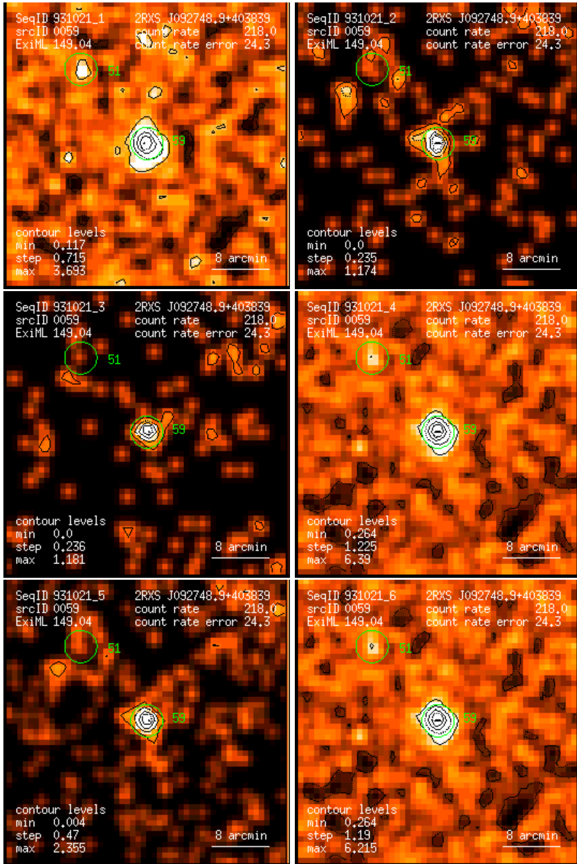
Figure 59: RASS 931021: detection 0059: band rate images, Gaussian filter: (1) PSPC channels 11 – 41, (2) 52 – 90, (3) 91 – 201, (4) 11 – 235, (5) 52 – 201, (6) 11 – 201. Broad band rates in counts/ks. Band rate contour levels in counts/ks/arcmin 2 .
