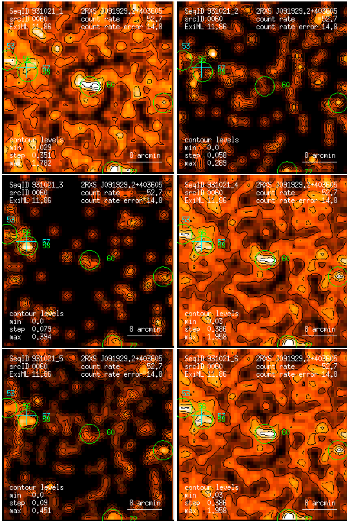
Figure 60: RASS 931021: detection 0060: band rate images, Gaussian filter: (1) PSPC channels 11 – 41, (2) 52 – 90, (3) 91 – 201, (4) 11 – 235, (5) 52 – 201, (6) 11 – 201. Broad band rates in counts/ks. Band rate contour levels in counts/ks/arcmin 2 .
