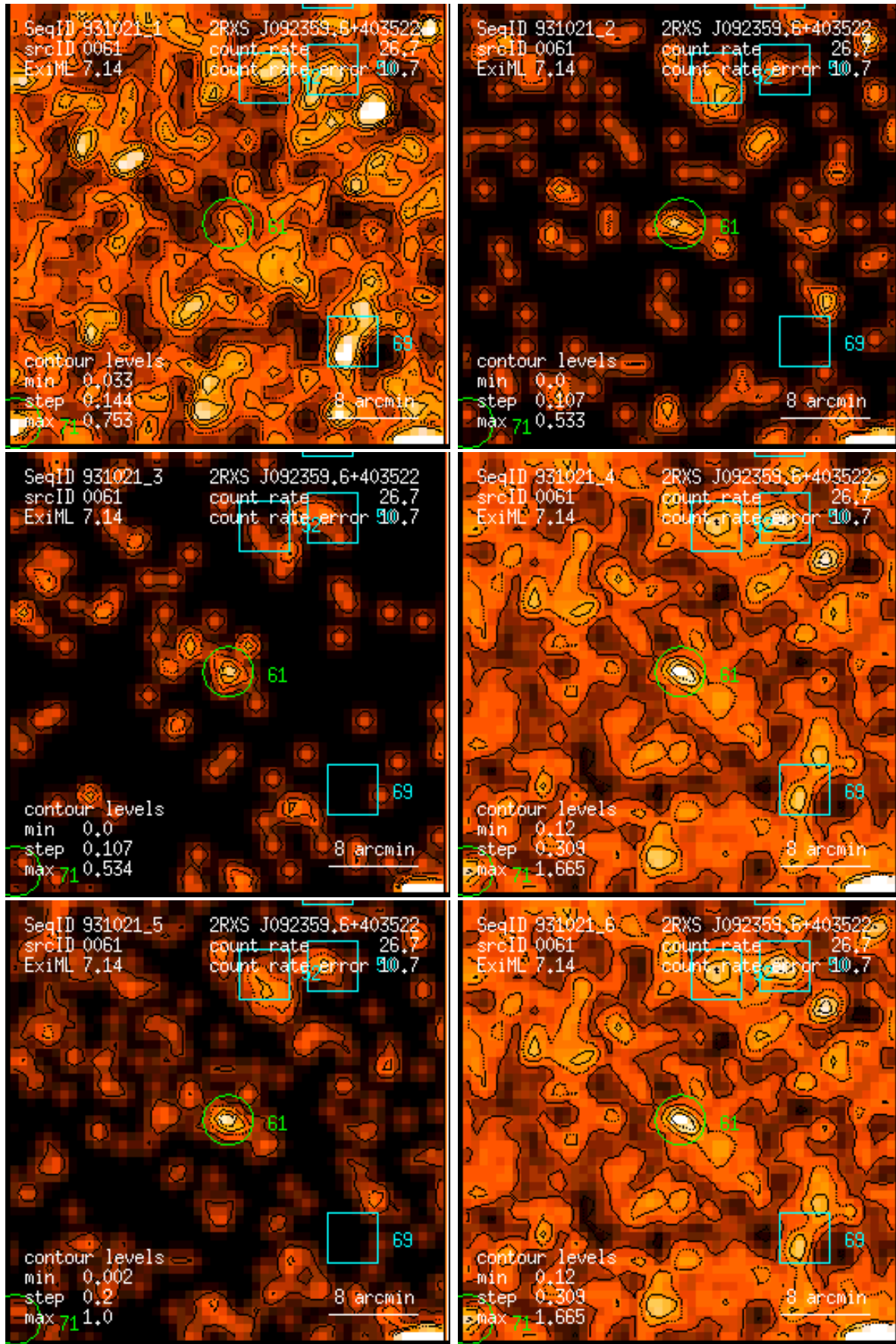
Figure 61: RASS 931021: detection 0061: band rate images, Gaussian filter: (1) PSPC channels 11 – 41, (2) 52 – 90, (3) 91 – 201, (4) 11 – 235, (5) 52 – 201, (6) 11 – 201. Broad band rates in counts/ks. Band rate contour levels in counts/ks/arcmin 2 .
