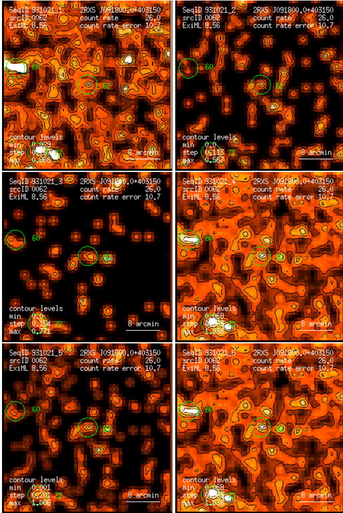
Figure 62: RASS 931021: detection 0062: band rate images, Gaussian filter: (1) PSPC channels 11 – 41, (2) 52 – 90, (3) 91 – 201, (4) 11 – 235, (5) 52 – 201, (6) 11 – 201. Broad band rates in counts/ks. Band rate contour levels in counts/ks/arcmin 2 .
