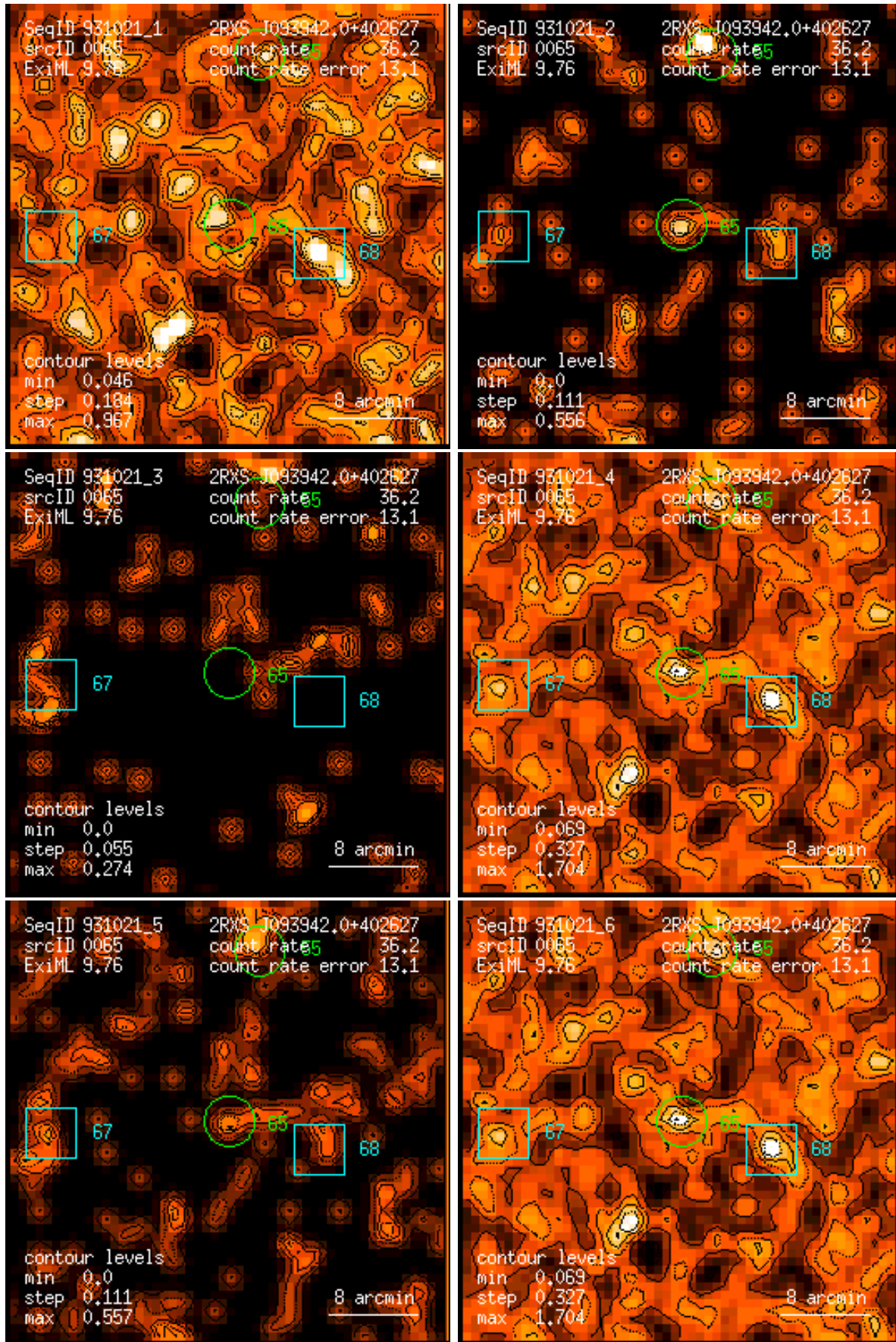
Figure 65: RASS 931021: detection 0065: band rate images, Gaussian filter: (1) PSPC channels 11 – 41, (2) 52 – 90, (3) 91 – 201, (4) 11 – 235, (5) 52 – 201, (6) 11 – 201. Broad band rates in counts/ks. Band rate contour levels in counts/ks/arcmin 2 .
