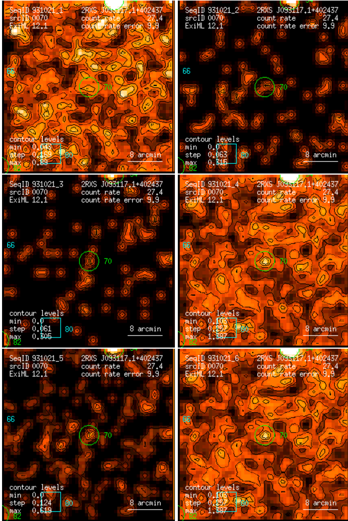
Figure 70: RASS 931021: detection 0070: band rate images, Gaussian filter: (1) PSPC channels 11 – 41, (2) 52 – 90, (3) 91 – 201, (4) 11 – 235, (5) 52 – 201, (6) 11 – 201. Broad band rates in counts/ks. Band rate contour levels in counts/ks/arcmin 2 .
