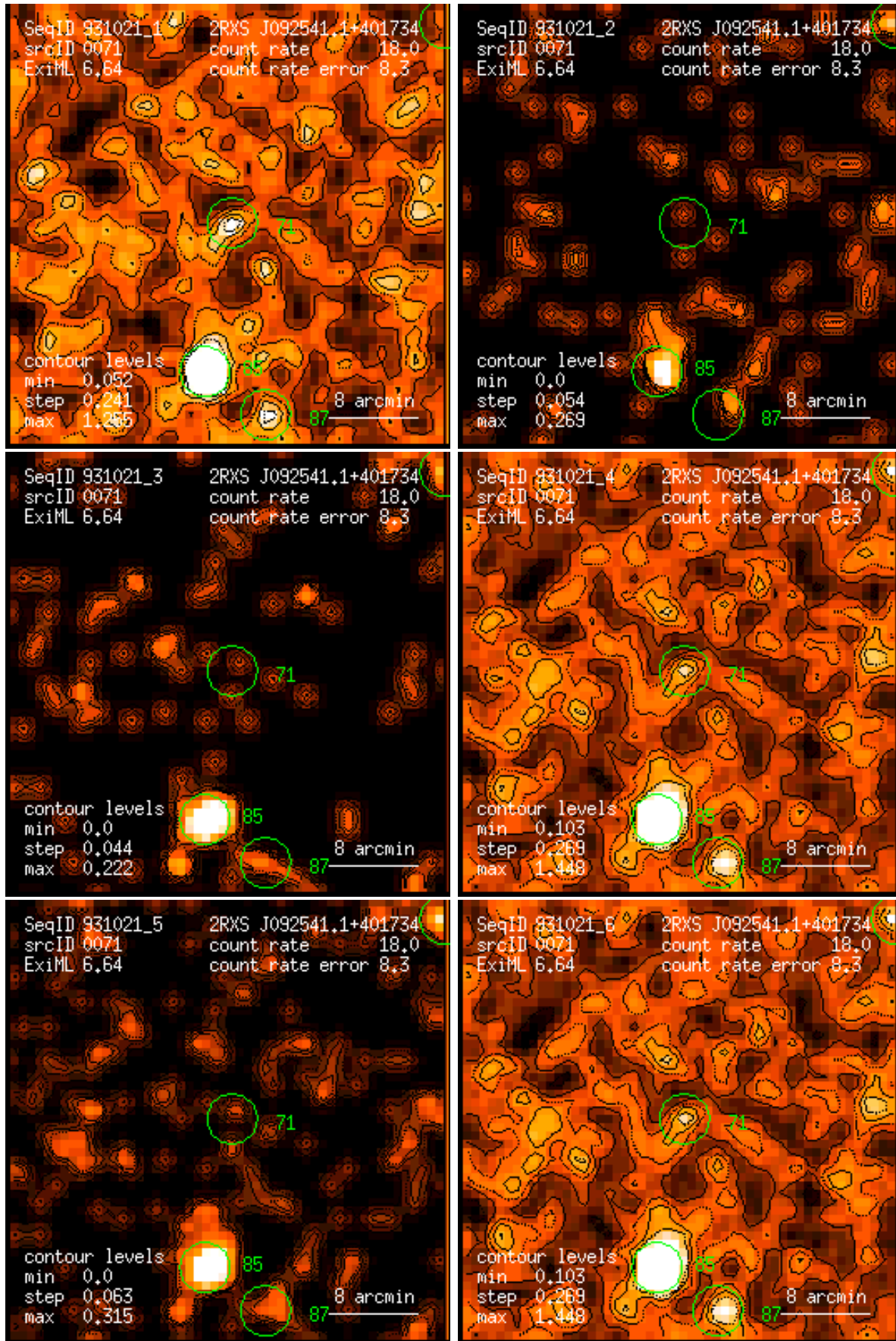
Figure 71: RASS 931021: detection 0071: band rate images, Gaussian filter: (1) PSPC channels 11 – 41, (2) 52 – 90, (3) 91 – 201, (4) 11 – 235, (5) 52 – 201, (6) 11 – 201. Broad band rates in counts/ks. Band rate contour levels in counts/ks/arcmin 2 .
