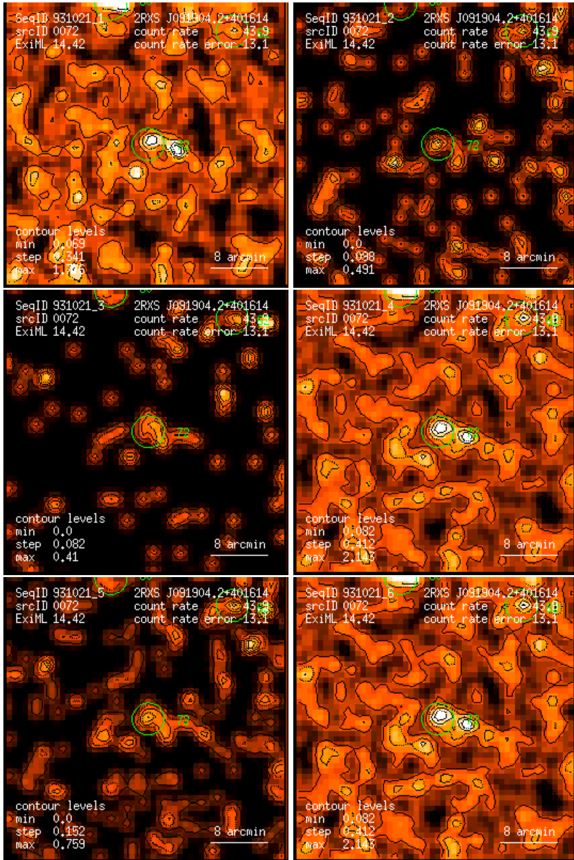
Figure 72: RASS 931021: detection 0072: band rate images, Gaussian filter: (1) PSPC channels 11 – 41, (2) 52 – 90, (3) 91 – 201, (4) 11 – 235, (5) 52 – 201, (6) 11 – 201. Broad band rates in counts/ks. Band rate contour levels in counts/ks/arcmin 2 .
