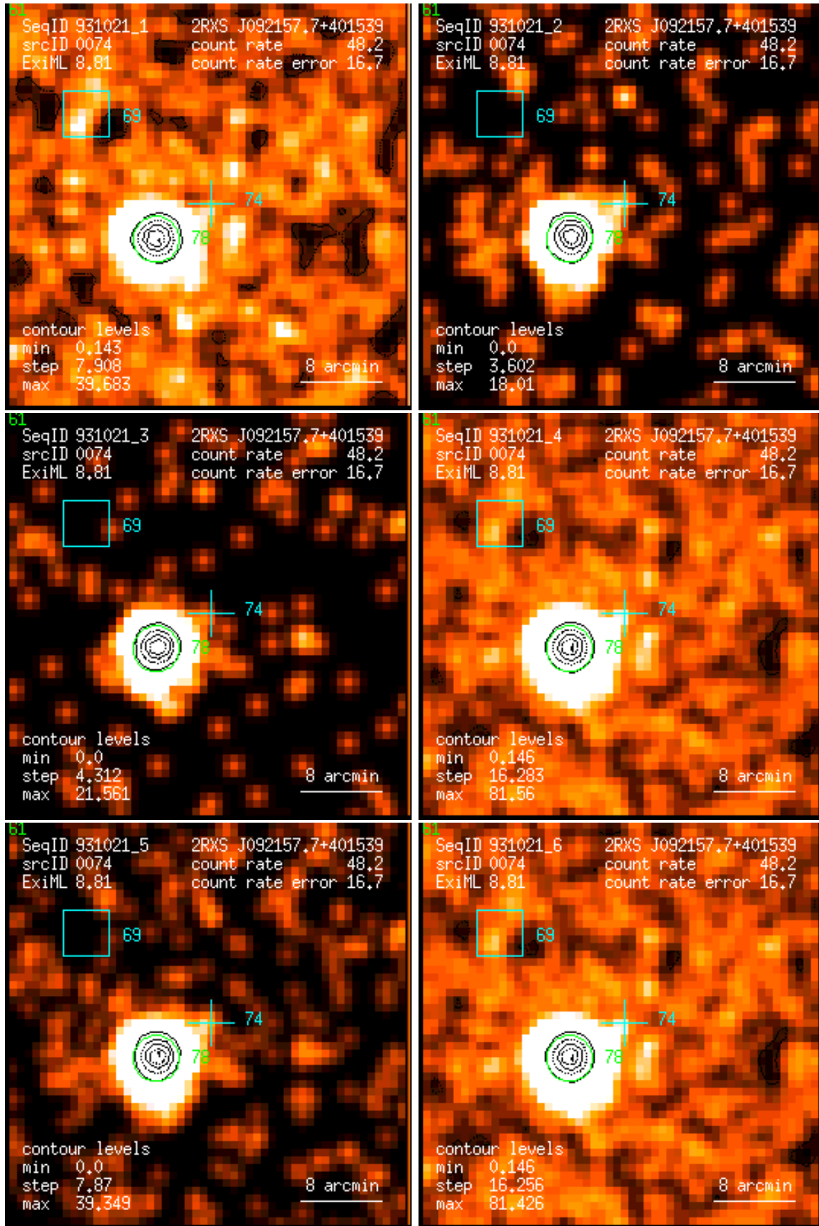
Figure 74: RASS 931021: detection 0074: band rate images, Gaussian filter: (1) PSPC channels 11 – 41, (2) 52 – 90, (3) 91 – 201, (4) 11 – 235, (5) 52 – 201, (6) 11 – 201. Broad band rates in counts/ks. Band rate contour levels in counts/ks/arcmin 2 .
