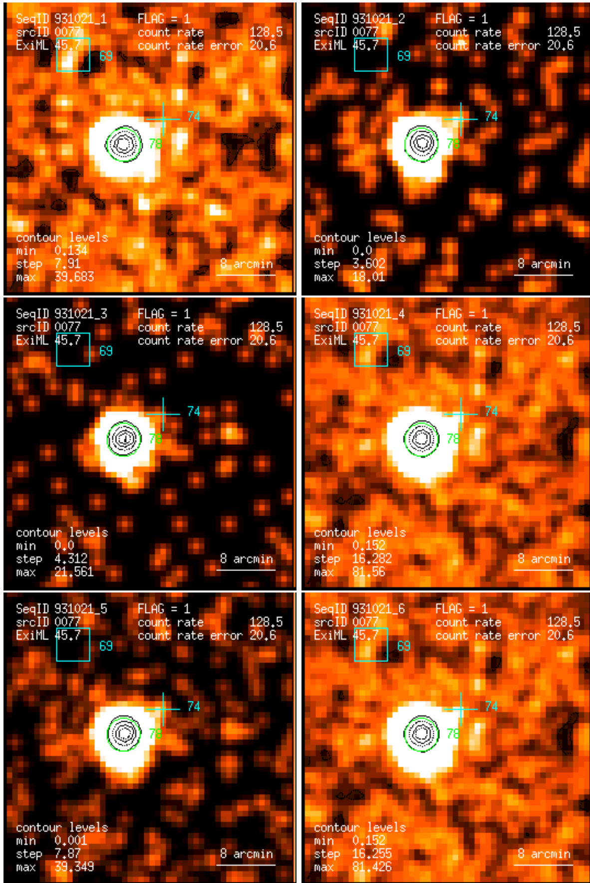
Figure 77: RASS 931021: detection 0077: band rate images, Gaussian filter: (1) PSPC channels 11 – 41, (2) 52 – 90, (3) 91 – 201, (4) 11 – 235, (5) 52 – 201, (6) 11 – 201. Broad band rates in counts/ks. Band rate contour levels in counts/ks/arcmin 2 .
