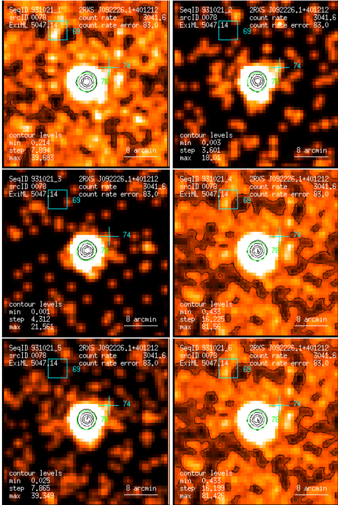
Figure 78: RASS 931021: detection 0078: band rate images, Gaussian filter: (1) PSPC channels 11 – 41, (2) 52 – 90, (3) 91 – 201, (4) 11 – 235, (5) 52 – 201, (6) 11 – 201. Broad band rates in counts/ks. Band rate contour levels in counts/ks/arcmin 2 .
