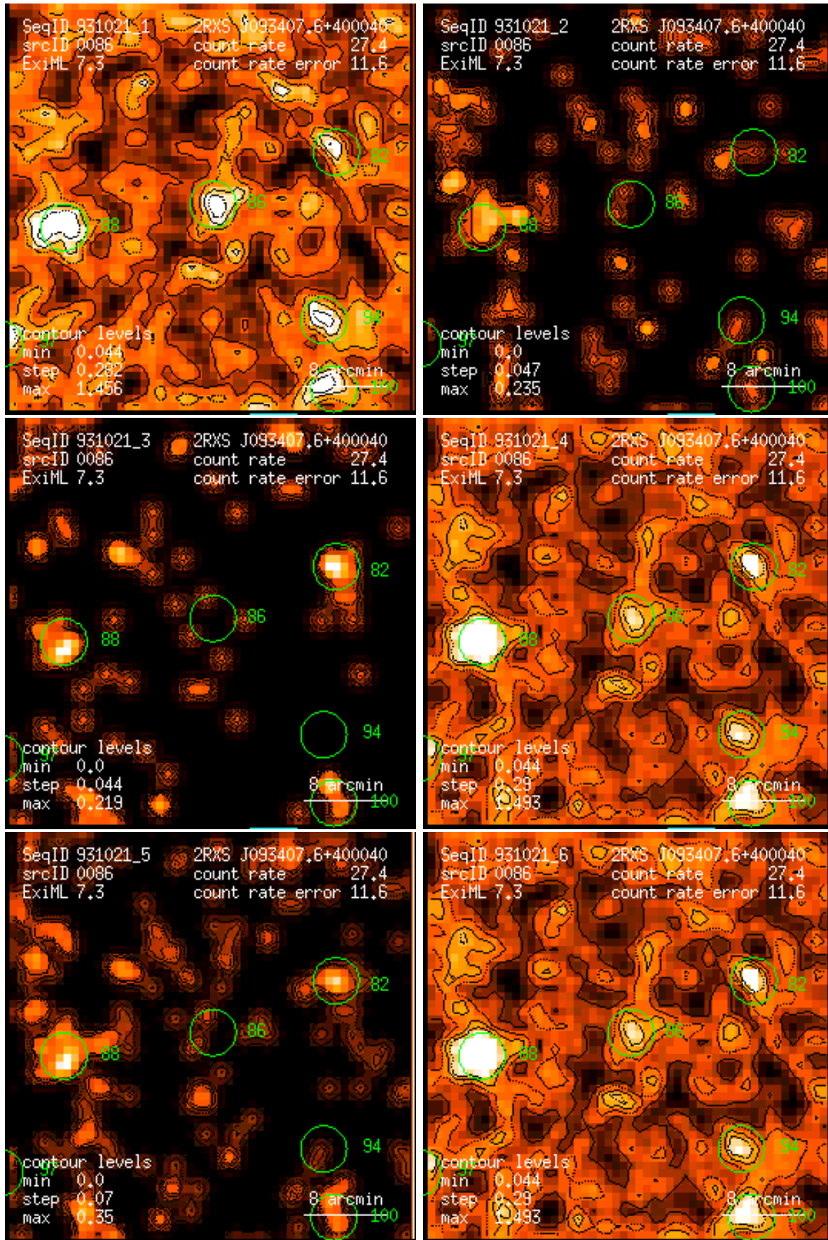
Figure 86: RASS 931021: detection 0086: band rate images, Gaussian filter: (1) PSPC channels 11 – 41, (2) 52 – 90, (3) 91 – 201, (4) 11 – 235, (5) 52 – 201, (6) 11 – 201. Broad band rates in counts/ks. Band rate contour levels in counts/ks/arcmin 2 .
