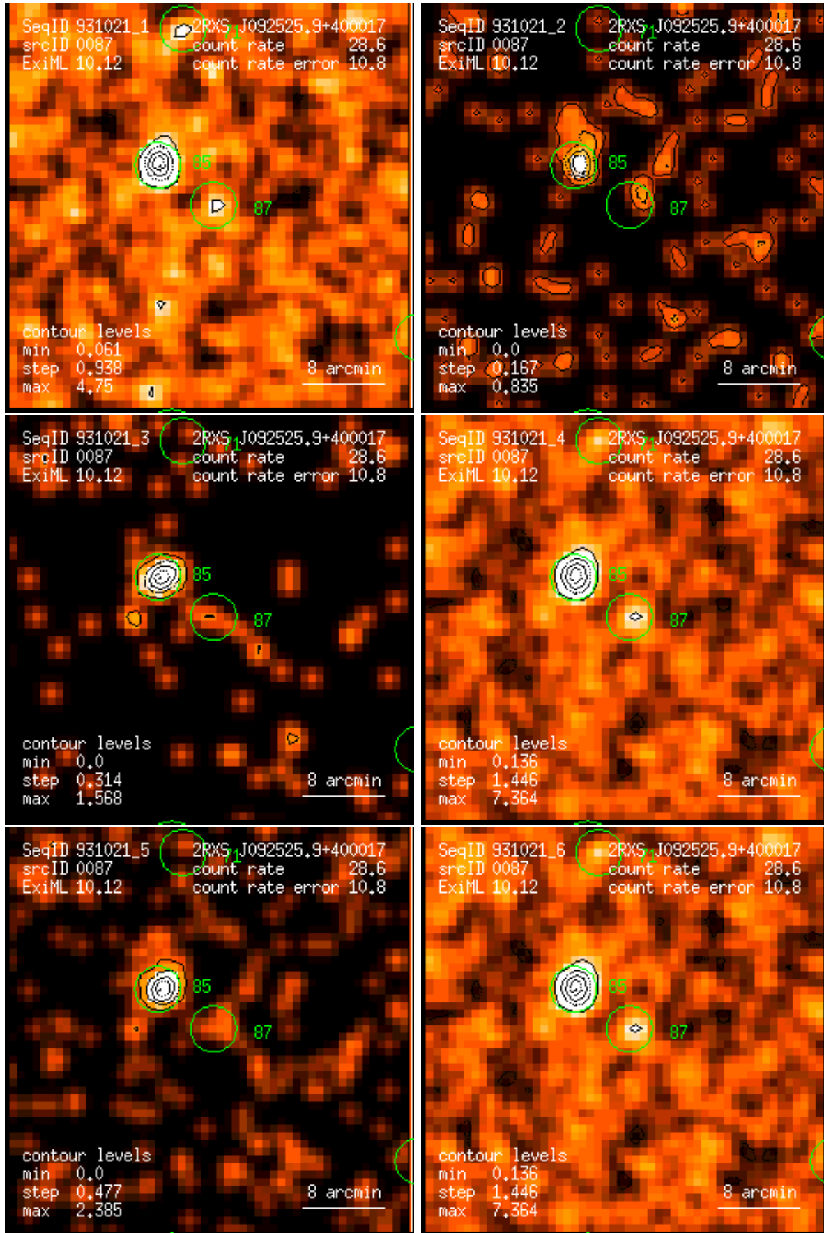
Figure 87: RASS 931021: detection 0087: band rate images, Gaussian filter: (1) PSPC channels 11 – 41, (2) 52 – 90, (3) 91 – 201, (4) 11 – 235, (5) 52 – 201, (6) 11 – 201. Broad band rates in counts/ks. Band rate contour levels in counts/ks/arcmin 2 .
