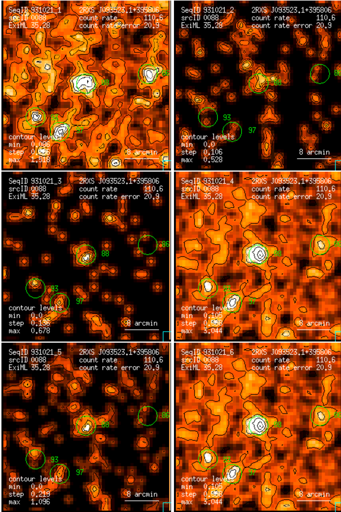
Figure 88: RASS 931021: detection 0088: band rate images, Gaussian filter: (1) PSPC channels 11 – 41, (2) 52 – 90, (3) 91 – 201, (4) 11 – 235, (5) 52 – 201, (6) 11 – 201. Broad band rates in counts/ks. Band rate contour levels in counts/ks/arcmin 2 .
