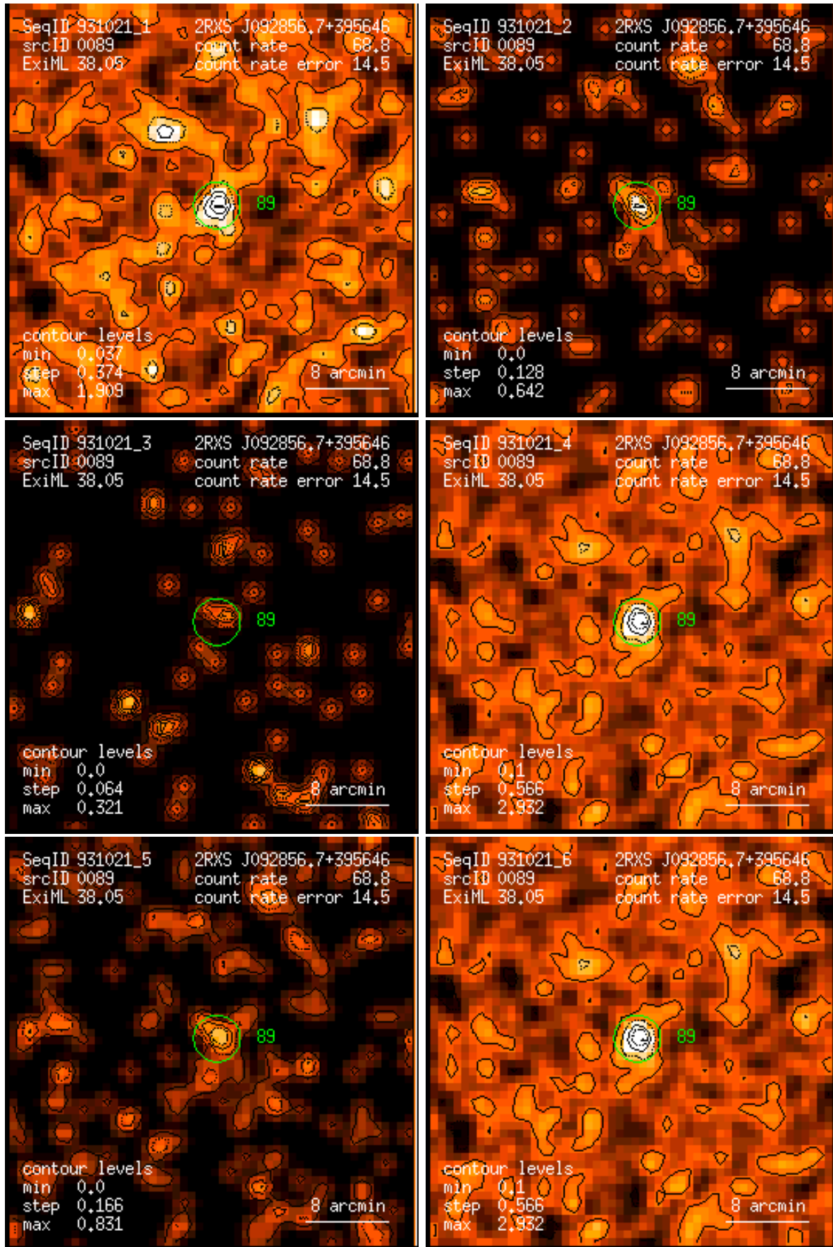
Figure 89: RASS 931021: detection 0089: band rate images, Gaussian filter: (1) PSPC channels 11 – 41, (2) 52 – 90, (3) 91 – 201, (4) 11 – 235, (5) 52 – 201, (6) 11 – 201. Broad band rates in counts/ks. Band rate contour levels in counts/ks/arcmin 2 .
