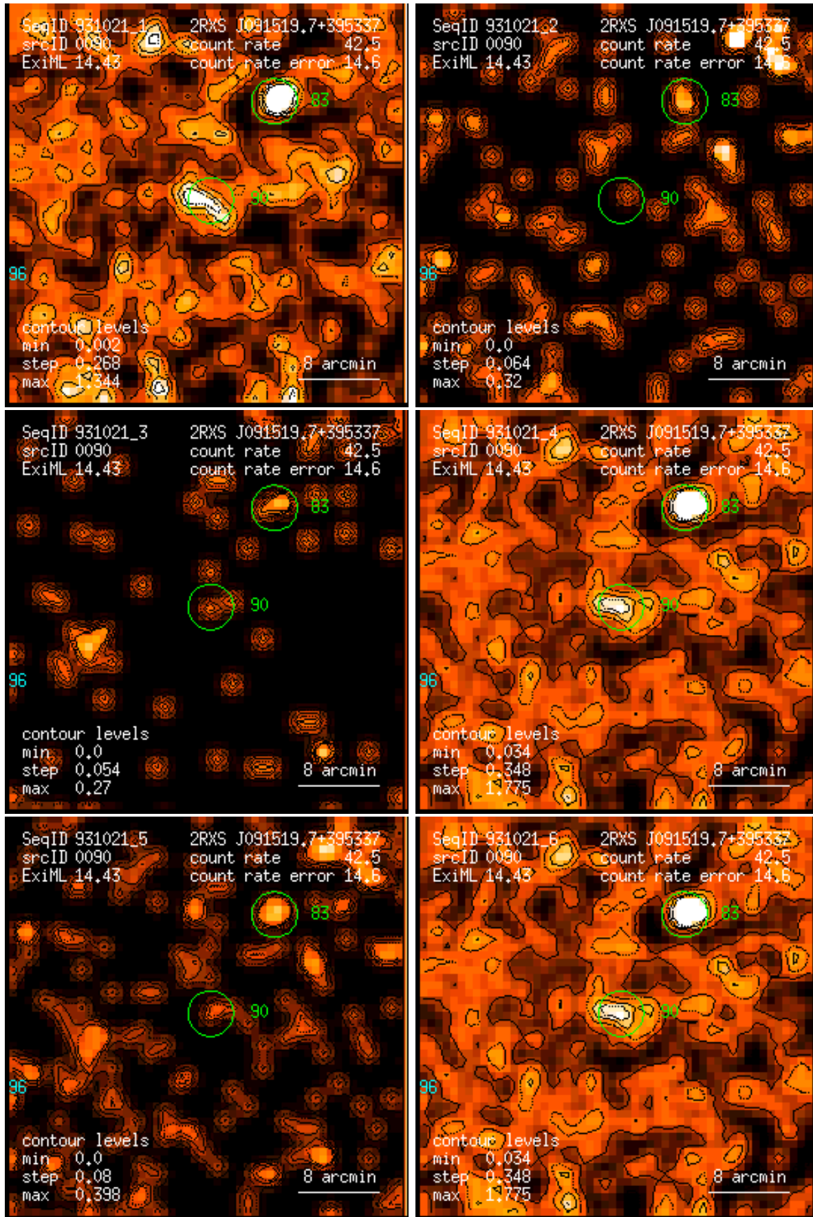
Figure 90: RASS 931021: detection 0090: band rate images, Gaussian filter: (1) PSPC channels 11 – 41, (2) 52 – 90, (3) 91 – 201, (4) 11 – 235, (5) 52 – 201, (6) 11 – 201. Broad band rates in counts/ks. Band rate contour levels in counts/ks/arcmin 2 .
