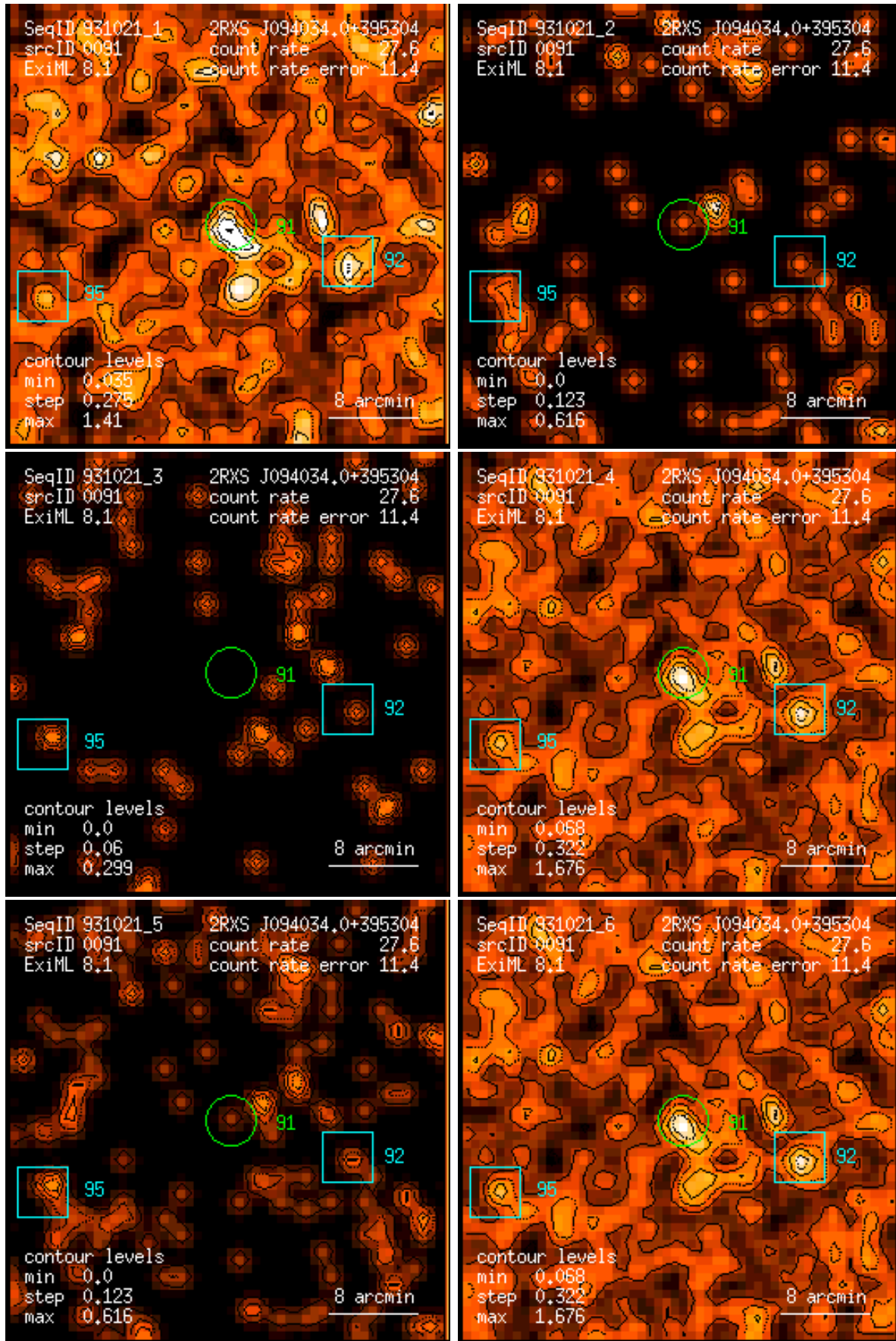
Figure 91: RASS 931021: detection 0091: band rate images, Gaussian filter: (1) PSPC channels 11 – 41, (2) 52 – 90, (3) 91 – 201, (4) 11 – 235, (5) 52 – 201, (6) 11 – 201. Broad band rates in counts/ks. Band rate contour levels in counts/ks/arcmin 2 .
