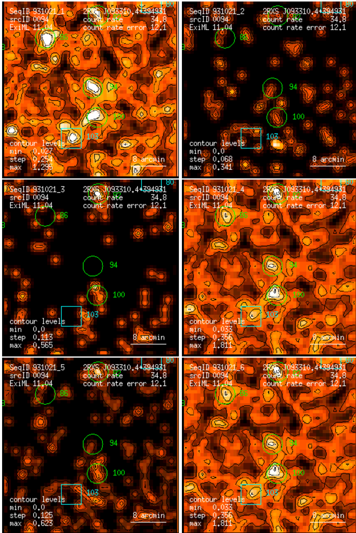
Figure 94: RASS 931021: detection 0094: band rate images, Gaussian filter: (1) PSPC channels 11 – 41, (2) 52 – 90, (3) 91 – 201, (4) 11 – 235, (5) 52 – 201, (6) 11 – 201. Broad band rates in counts/ks. Band rate contour levels in counts/ks/arcmin 2 .
