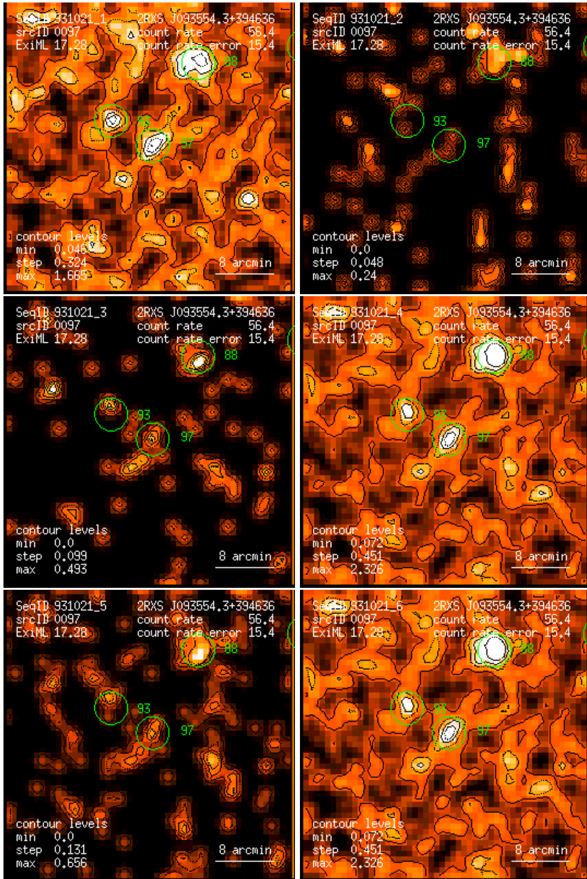
Figure 97: RASS 931021: detection 0097: band rate images, Gaussian filter: (1) PSPC channels 11 – 41, (2) 52 – 90, (3) 91 – 201, (4) 11 – 235, (5) 52 – 201, (6) 11 – 201. Broad band rates in counts/ks. Band rate contour levels in counts/ks/arcmin 2 .
