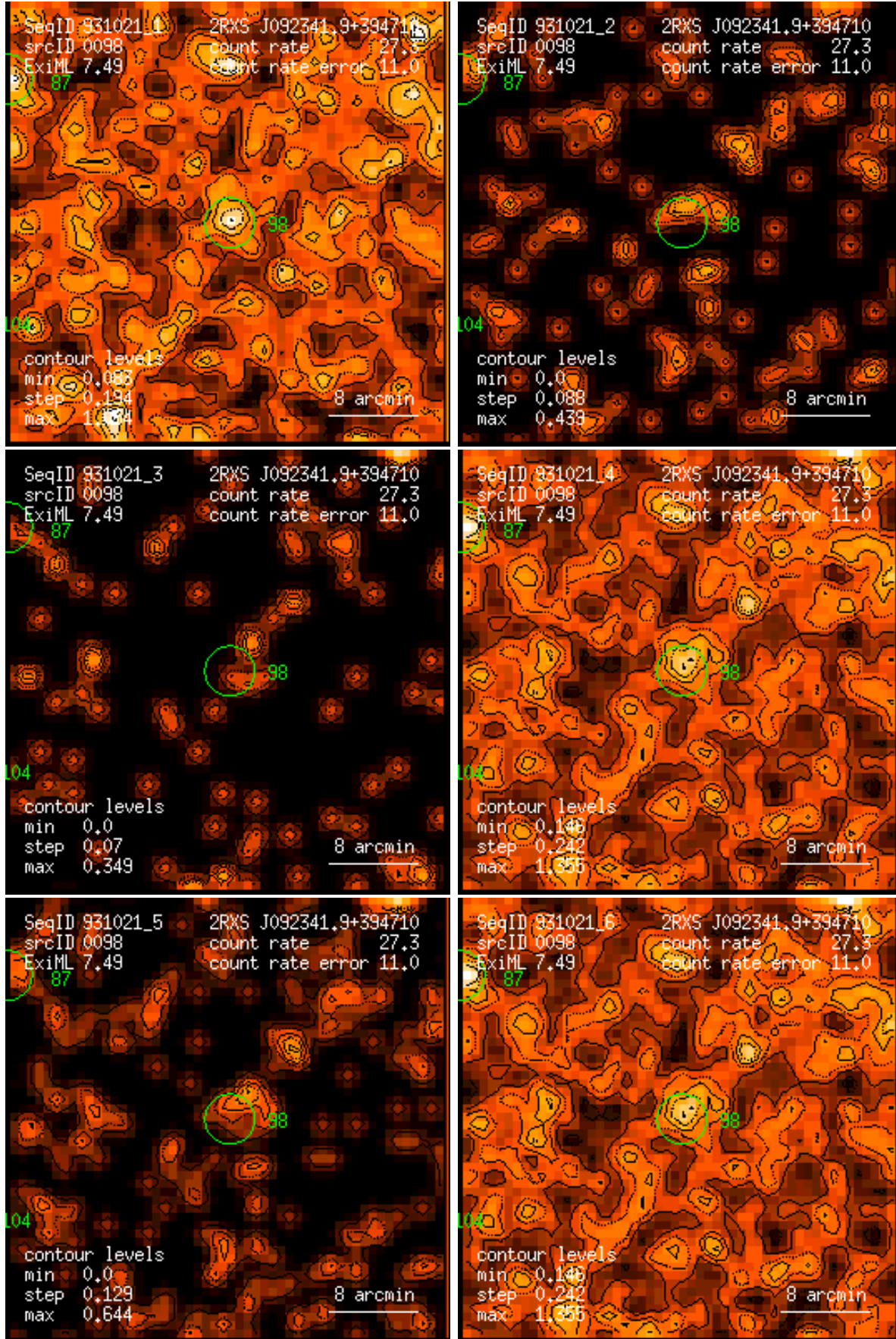
Figure 98: RASS 931021: detection 0098: band rate images, Gaussian filter: (1) PSPC channels 11 – 41, (2) 52 – 90, (3) 91 – 201, (4) 11 – 235, (5) 52 – 201, (6) 11 – 201. Broad band rates in counts/ks. Band rate contour levels in counts/ks/arcmin 2 .
