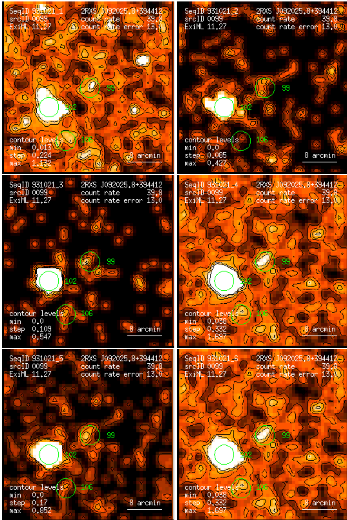
Figure 99: RASS 931021: detection 0099: band rate images, Gaussian filter: (1) PSPC channels 11 – 41, (2) 52 – 90, (3) 91 – 201, (4) 11 – 235, (5) 52 – 201, (6) 11 – 201. Broad band rates in counts/ks. Band rate contour levels in counts/ks/arcmin 2 .
