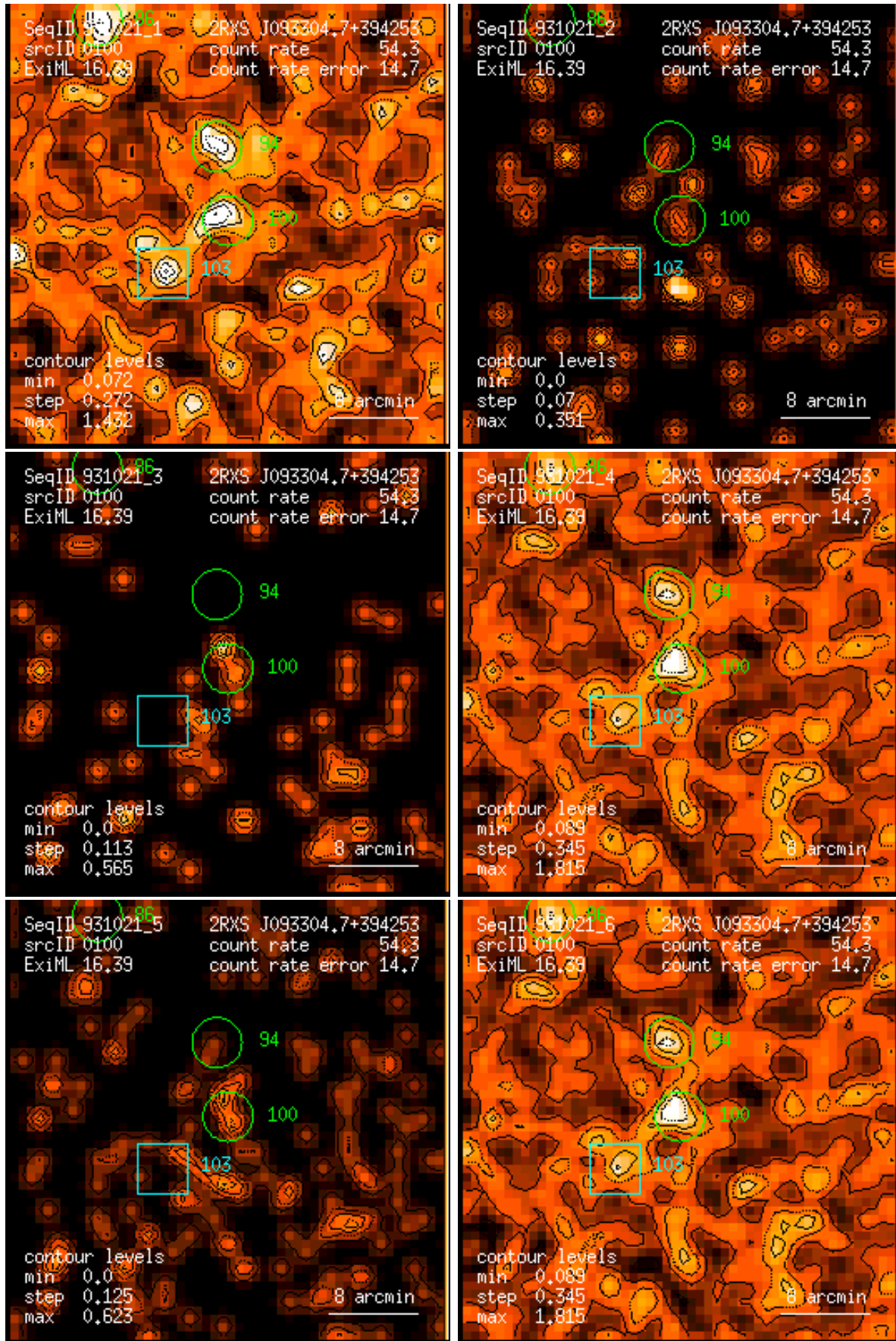
Figure 100: RASS 931021: detection 0100: band rate images, Gaussian filter: (1) PSPC channels 11 – 41, (2) 52 – 90, (3) 91 – 201, (4) 11 – 235, (5) 52 – 201, (6) 11 – 201. Broad band rates in counts/ks. Band rate contour levels in counts/ks/arcmin 2 .
