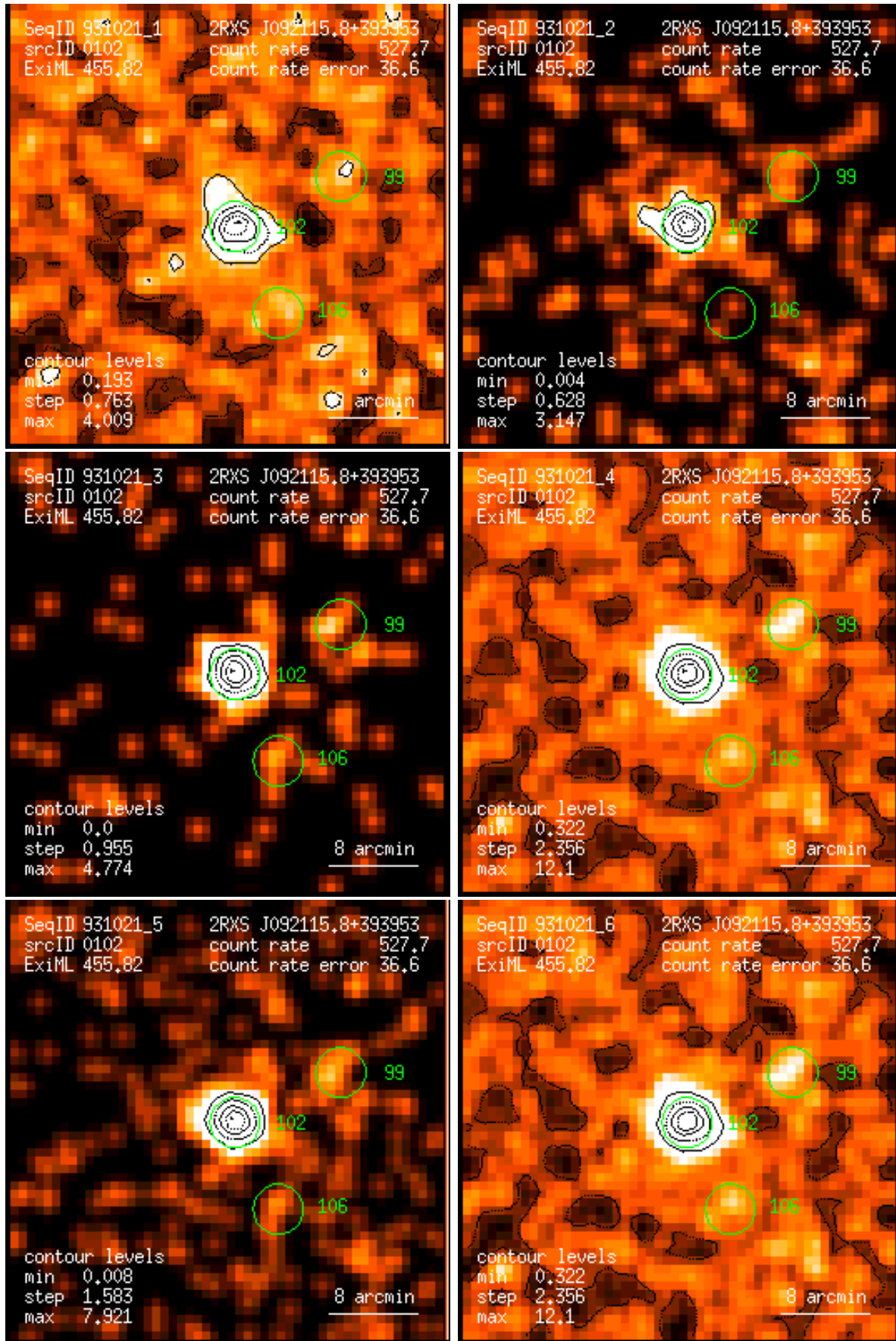
Figure 102: RASS 931021: detection 0102: band rate images, Gaussian filter: (1) PSPC channels 11 – 41, (2) 52 – 90, (3) 91 – 201, (4) 11 – 235, (5) 52 – 201, (6) 11 – 201. Broad band rates in counts/ks. Band rate contour levels in counts/ks/arcmin 2 .
