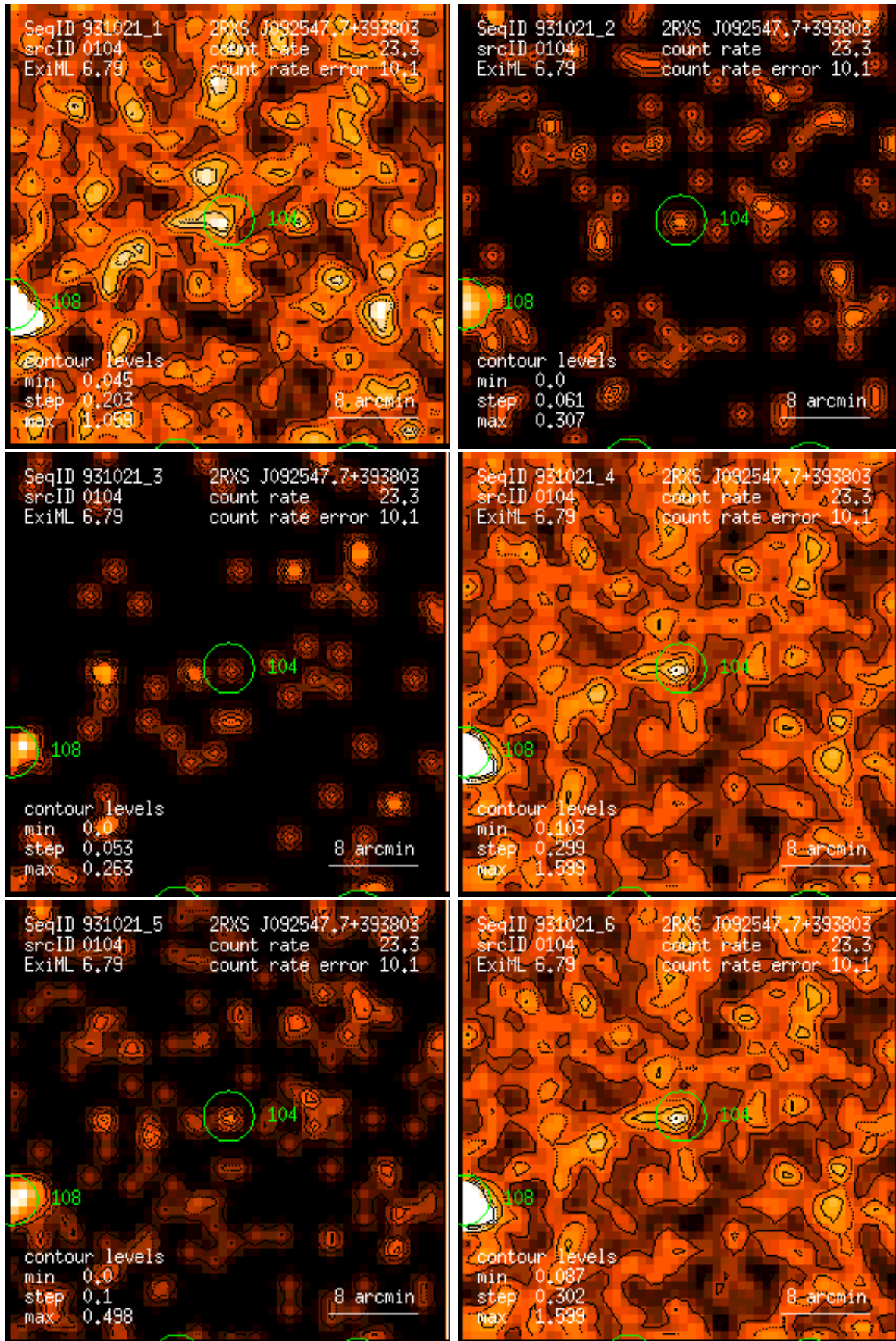
Figure 104: RASS 931021: detection 0104: band rate images, Gaussian filter: (1) PSPC channels 11 – 41, (2) 52 – 90, (3) 91 – 201, (4) 11 – 235, (5) 52 – 201, (6) 11 – 201. Broad band rates in counts/ks. Band rate contour levels in counts/ks/arcmin 2 .
