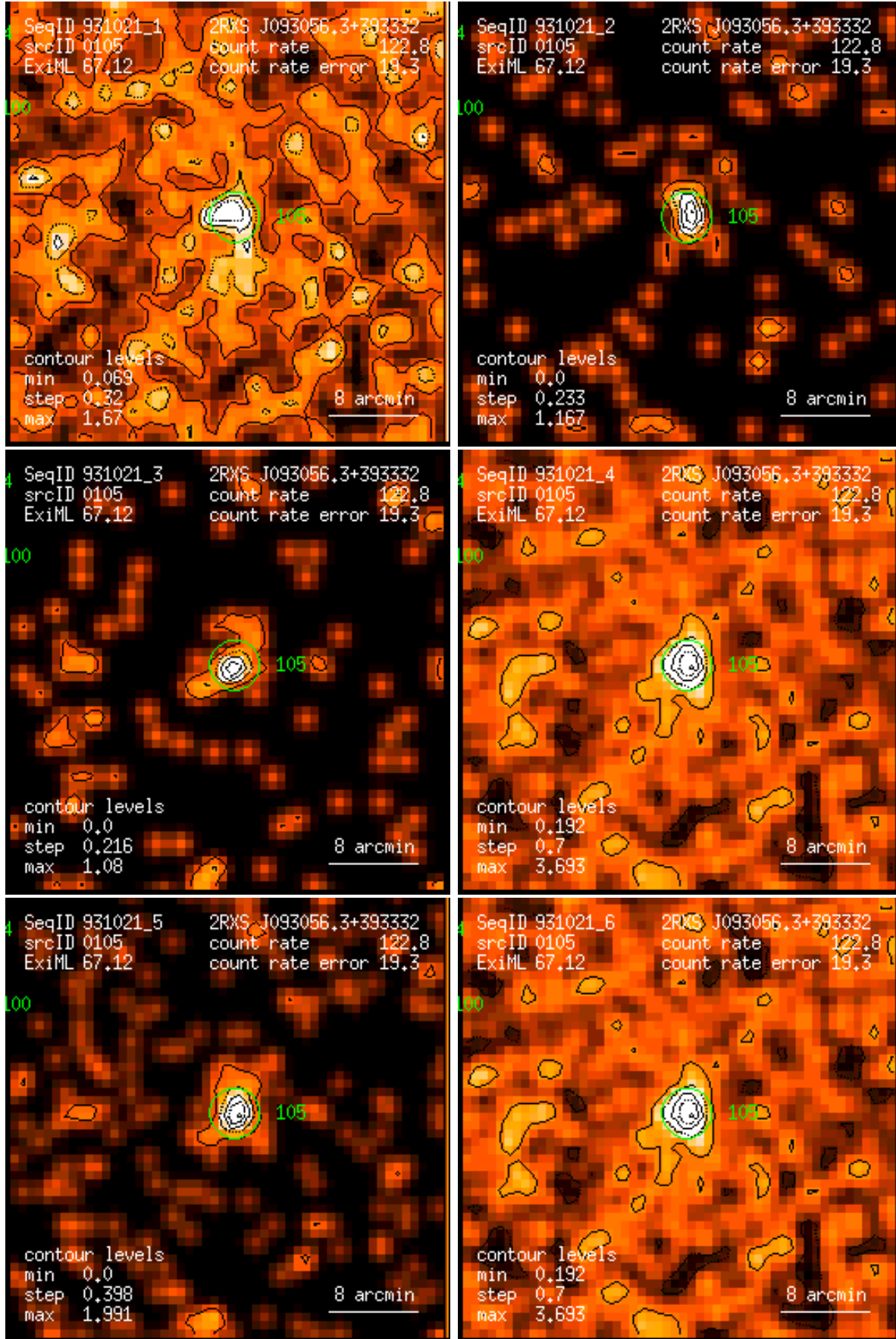
Figure 105: RASS 931021: detection 0105: band rate images, Gaussian filter: (1) PSPC channels 11 – 41, (2) 52 – 90, (3) 91 – 201, (4) 11 – 235, (5) 52 – 201, (6) 11 – 201. Broad band rates in counts/ks. Band rate contour levels in counts/ks/arcmin 2 .
