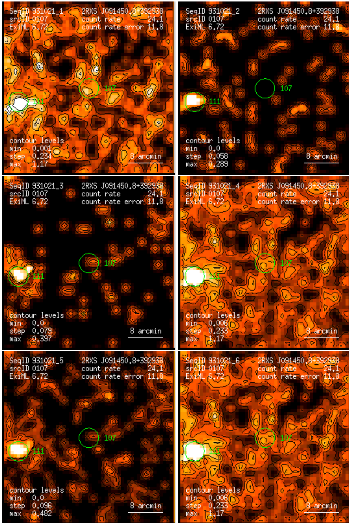
Figure 107: RASS 931021: detection 0107: band rate images, Gaussian filter: (1) PSPC channels 11 – 41, (2) 52 – 90, (3) 91 – 201, (4) 11 – 235, (5) 52 – 201, (6) 11 – 201. Broad band rates in counts/ks. Band rate contour levels in counts/ks/arcmin 2 .
